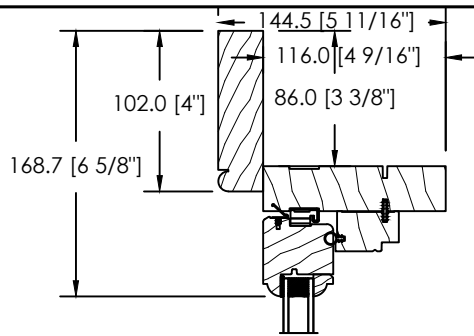
DS-001 BRICKMOULD
