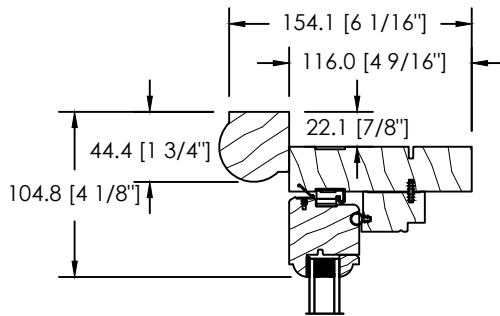
DS-030 BRICKMOULD
