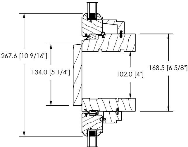
4" SPACE MULL OR STUD POCKET
