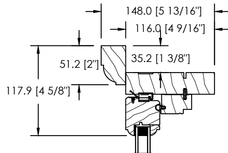
DS-034 BRICKMOULD
