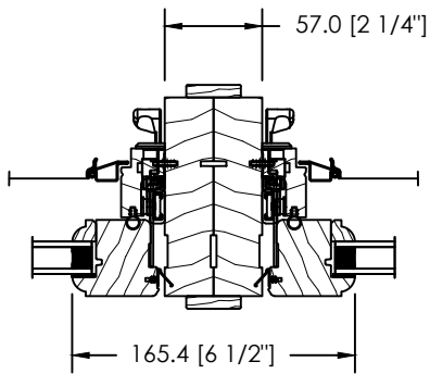
2 WIDE OPERATING STANDARD MODULAR MULL
