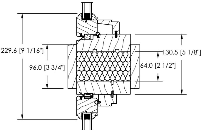
2 1/2" INSULATED SPACE MULL OR STUD POCKET
