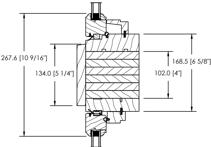
4" SOLID SPACE MULL OR STUD POCKET
