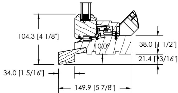
STANDARD 1 1/4" SILL NOSING GB-021
