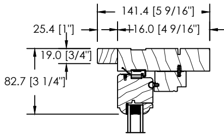
FLUSH 1" EXTERIOR EXTENSION
