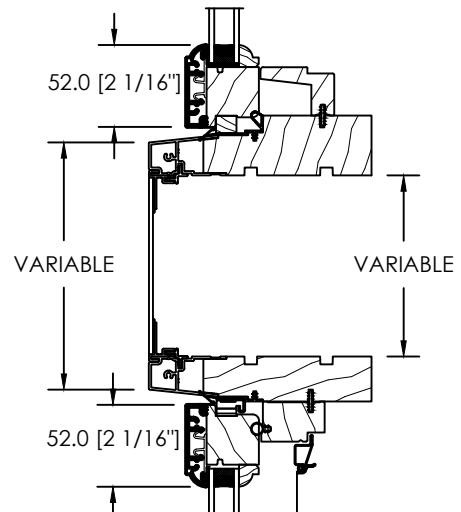
CUSTOM SPACE MULL OR STUD POCKET 8" MAXIMUM
