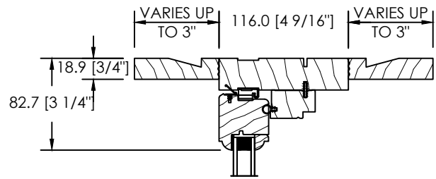
FLUSH UP TO 3" EXT. AND INT. EXTENSION
