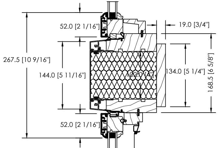
4" INSULATED SPACE MULL OR STUD POCKET
