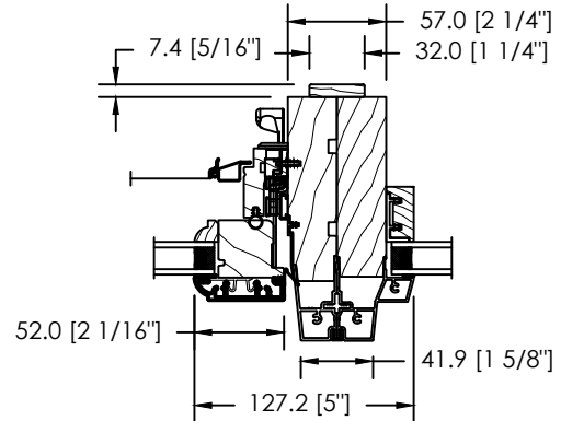
OPERATING, DIRECT SET MODULAR MULL
