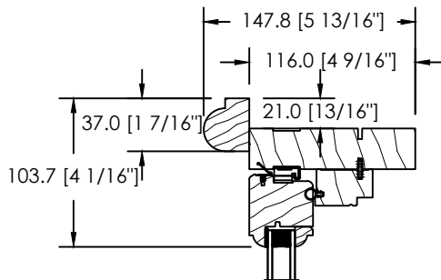
DS-034 BRICKMOULD
