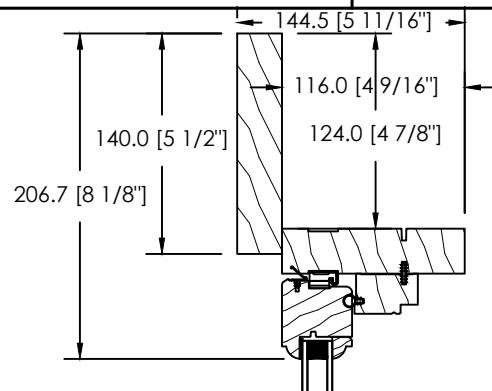
5/4 X 5 1/2" FLAT CASING
