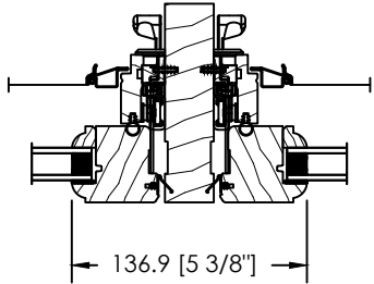
2 WIDE OPERATING STANDARD STRUCTURAL MULL
