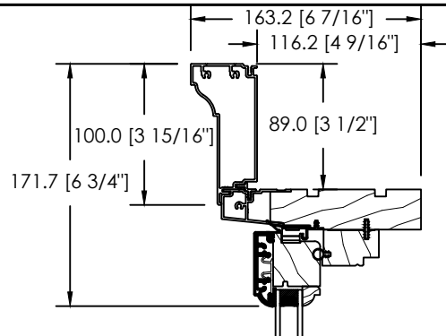
ALUMINIUM CLAD BACK BEND BRICKMOULD D-090
