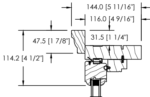
COLONIAL EXTERIOR BRICKMOULD
