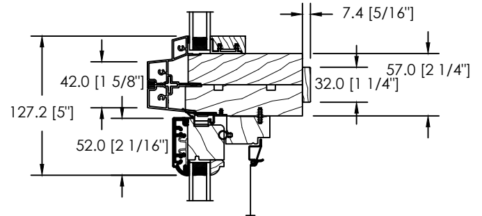
DIRECT SET OVER OPERATING TIGHT MULL
