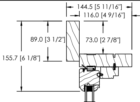
5/4 X 3 1/2" FLAT CASING
