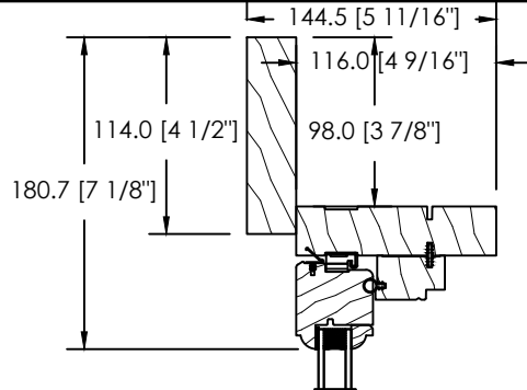
5/4 X 4 1/2" FLAT CASING
