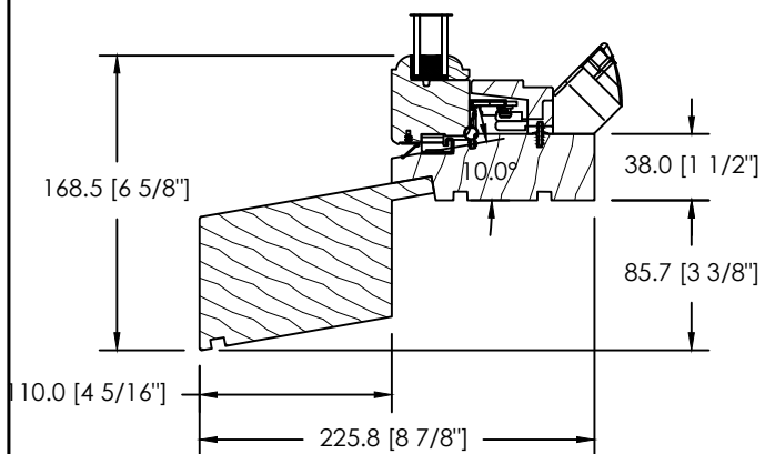
DS-072 SILL NOSING
