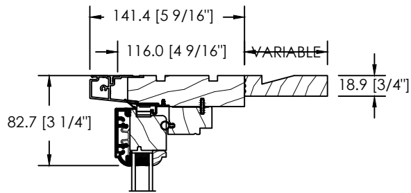
INTERIOR EXTENSION
