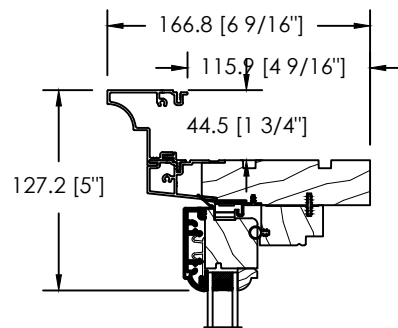
ALUMINIUM CLAD SKYLER BRICKMOULD D-174
