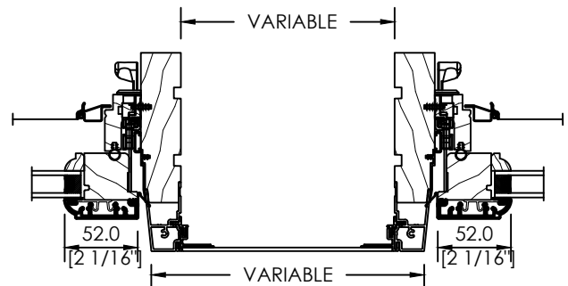
CUSTOM SPACE MULL OR STUD POCKET 8" MAXIMUM
