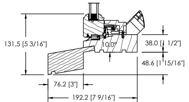
LONG HISTORIC SILL NOSING GB-058
