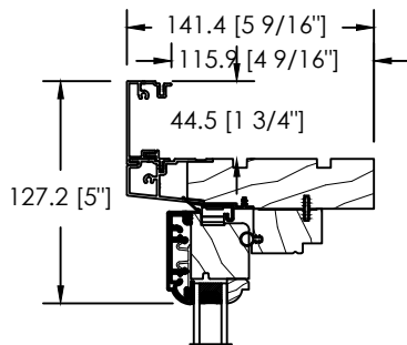
ALUMINIUM CLAD 1 3/4" FLAT BRICKMOULD D-116
