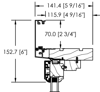
ALUMINIUM CLAD 2 3/4" FLAT BRICKMOULD D-066
