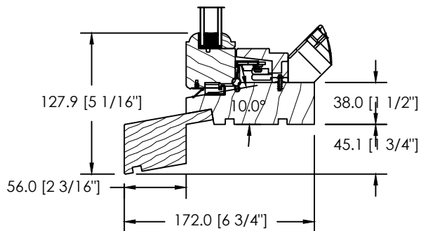
HISTORIC SILL NOSING GB-036
