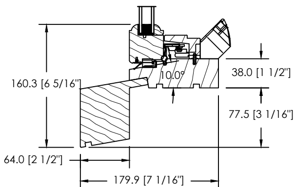
DS-073 SILL NOSING
