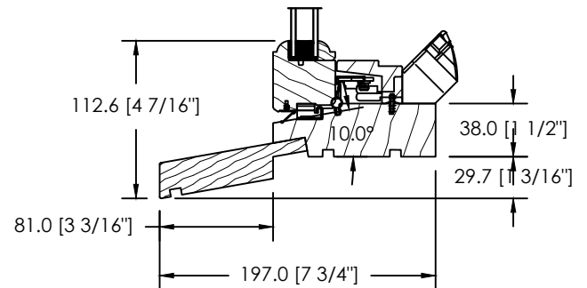
3" LONG SILL NOSING GB-040
