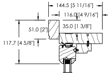
DS-031 BRICKMOULD
