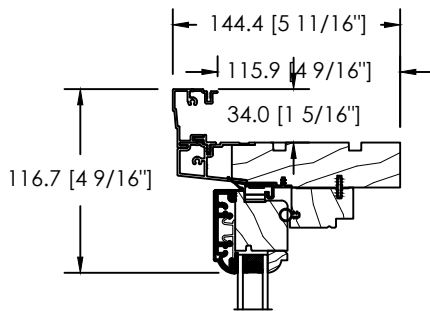
ALUMINIUM CLAD 908 BRICKMOULD
