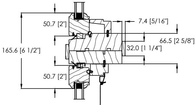
FIXED OVER OPERATING TIGHT MULL
