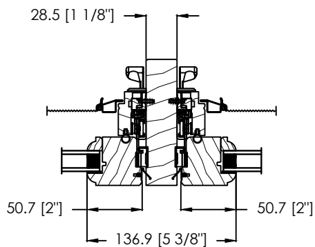
2 WIDE OPERATING STANDARD STRUCTURAL MULL
