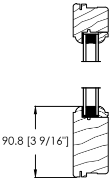
COLONIAL SASH & GLASS STOP-WIDE BOTTOM RAIL
