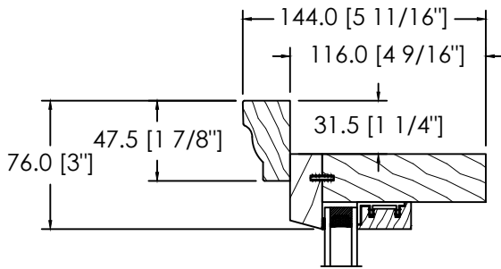
COLONIAL EXTERIOR BRICKMOULD D-017
