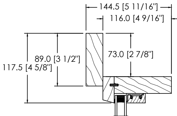
5/4 X 3 1/2" FLAT CASING D-061
