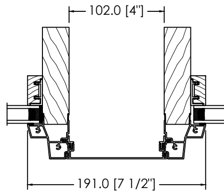
4" STUD POCKET OR SPACE MULL
