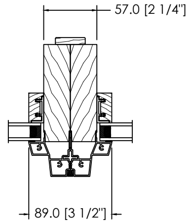
STANDARD HORIZONTAL MODULAR MULL
