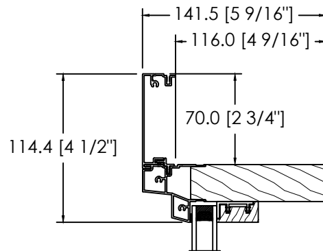
ALUMINIUM CLAD 2 3/4" FLAT BRICKMOULD D-066
