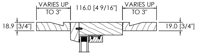
FLUSH UP TO 3" EXT. AND INT. EXTENSION
