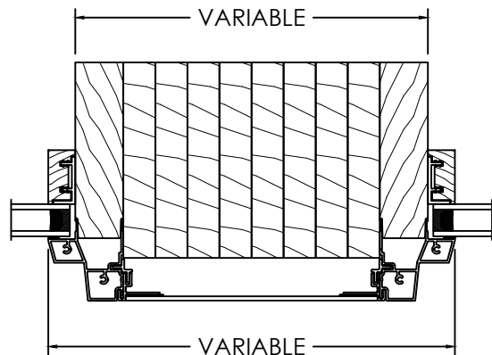
VARIABLE SOLID STUD POCKET OR SPACE MULL
