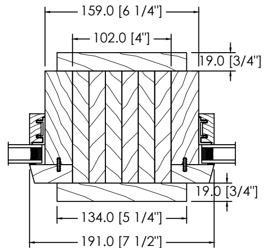
4" SOLID STUD POCKET OR SPACE MULL
