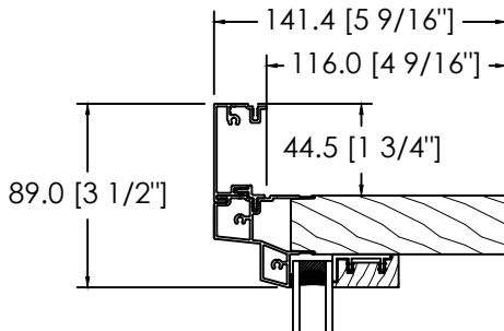
ALUMINIUM CLAD 1 3/4" FLAT BRICKMOULD D-116
