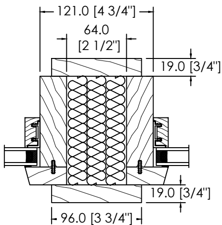
2 1/2" INSULATED STUD POCKET OR SPACE MULL
