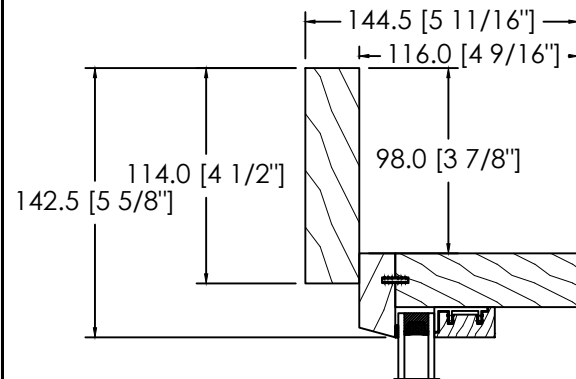
5/4 X 4 1/2" FLAT CASING D-117
