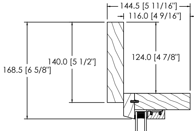
5/4 X 5 1/2" FLAT CASING D-118
