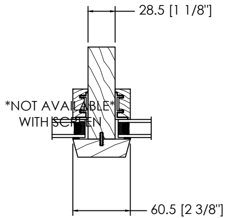
STANDARD HORIZONTAL STRUCTURAL MULL
