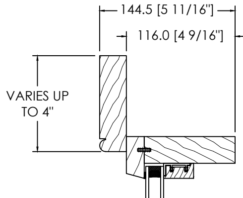
VARIABLE BRICKMOULD DS-001
