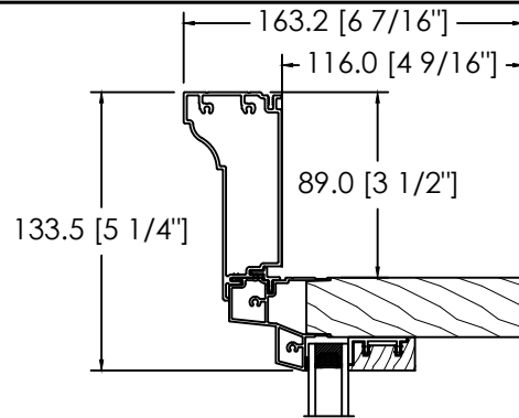
ALUMINIUM CLAD BACK BEND BRICKMOULD D-090
