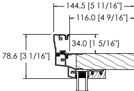
ALUMINIUM CLAD 908 BRICKMOULD D-065
