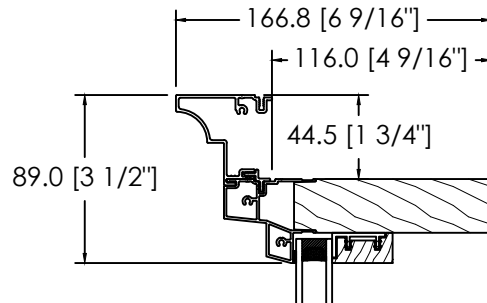
ALUMINIUM CLAD SKYLER BRICKMOULD D-174
