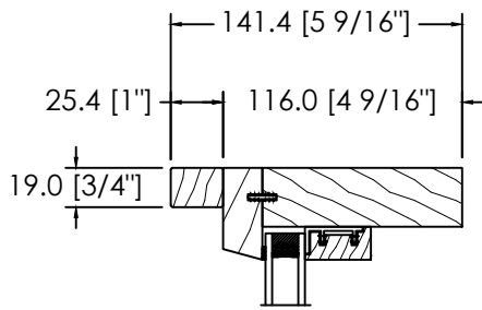
FLUSH 1" EXTERIOR EXTENSION
