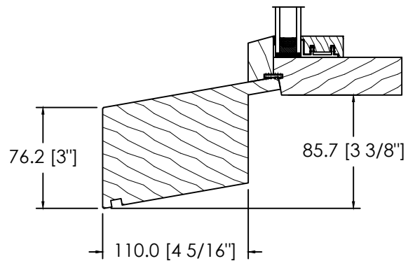
SPECIAL SILL EXTENSION (DS-072)
