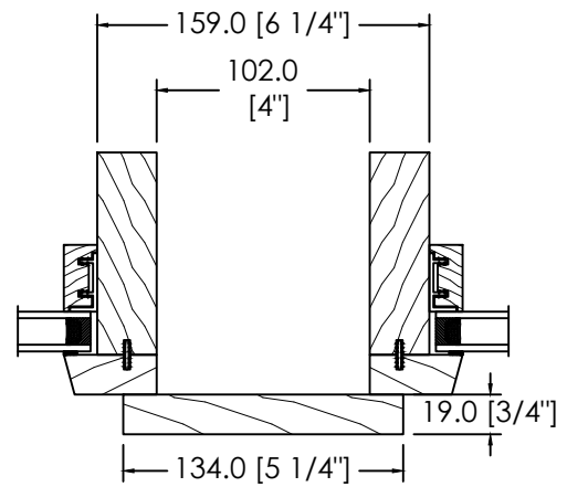
4" STUD POCKET OR SPACE MULL
