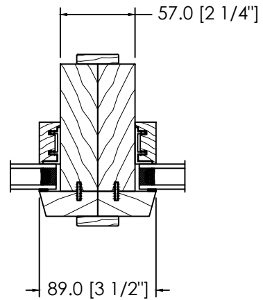
STANDARD HORIZONTAL MODULAR MULL
