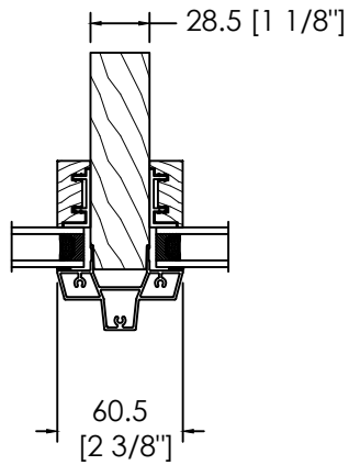
STANDARD HORIZONTAL STRUCTURAL MULL
