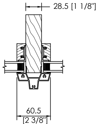
ASSEMBLAGE HORIZONTAL STRUCTURAL
