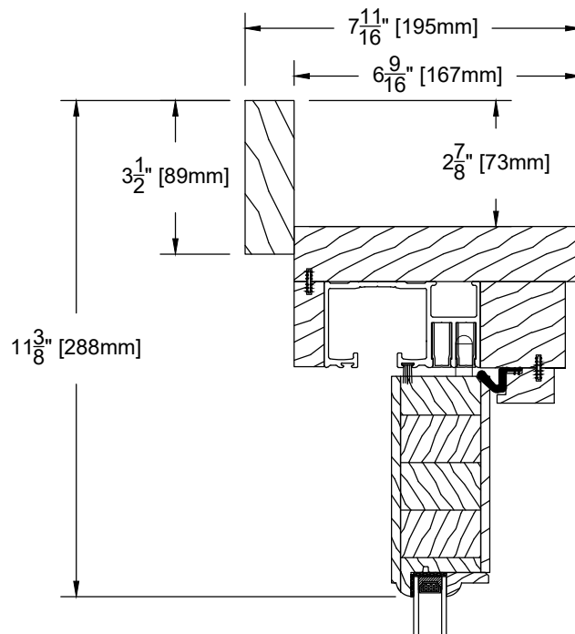
3 1/2" FLAT CASING
