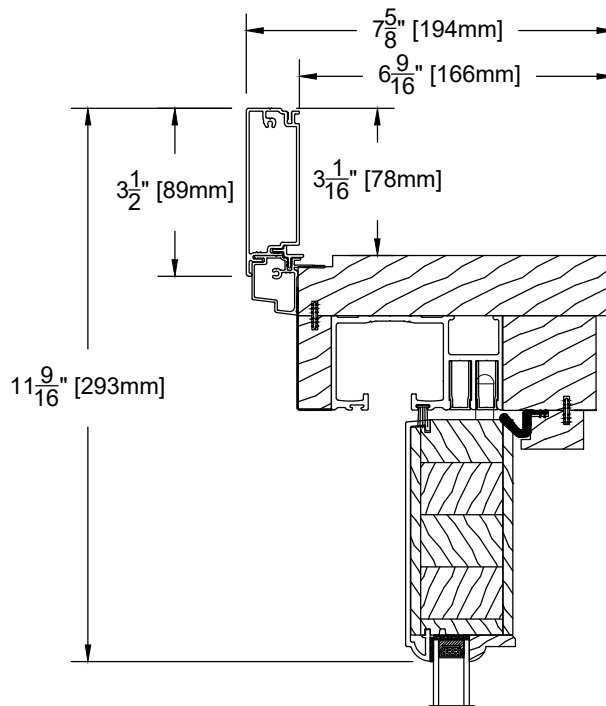
3 1/2" FLAT CASING (D-050)
