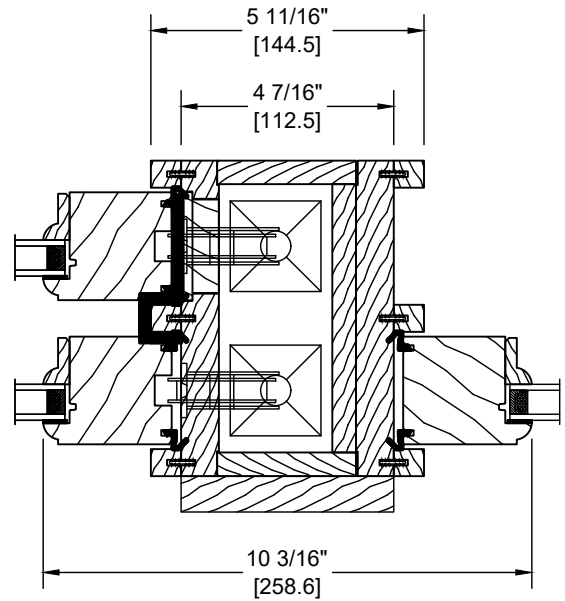
OPERATING WITH FIXED SASH MODULAR MULL
