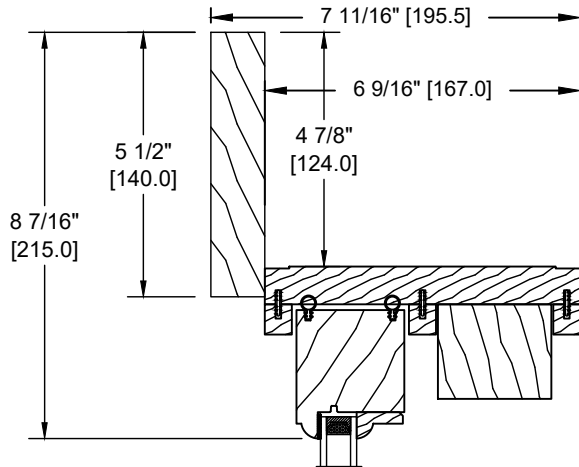
5/4 X 5 1/2" FLAT CASING (D-118)
