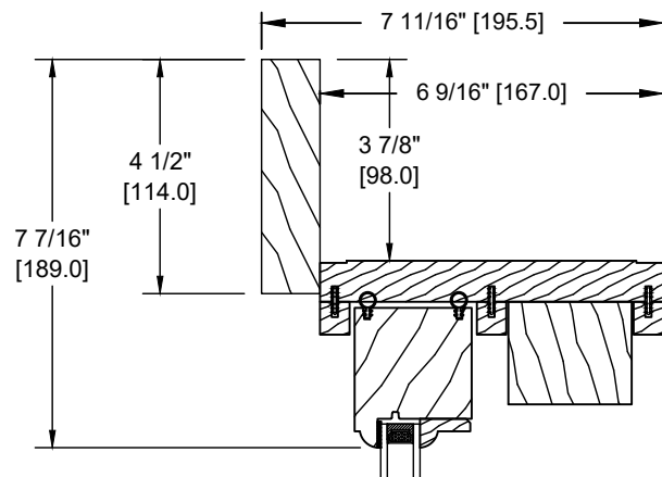
5/4 X 4 1/2" FLAT CASING (D-117)
