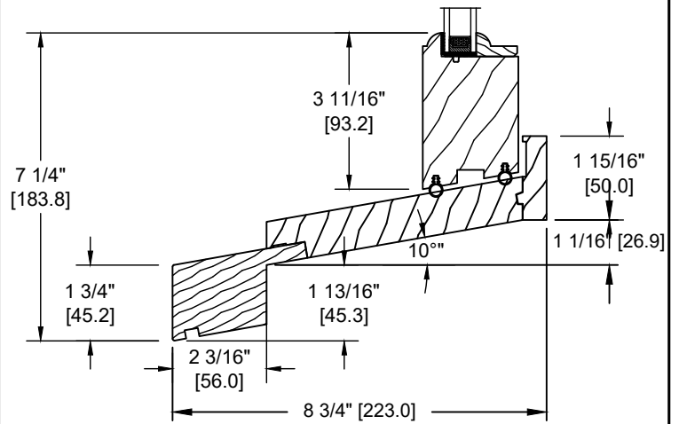
HISTORIC SILL EXTENSION (GB-036)
