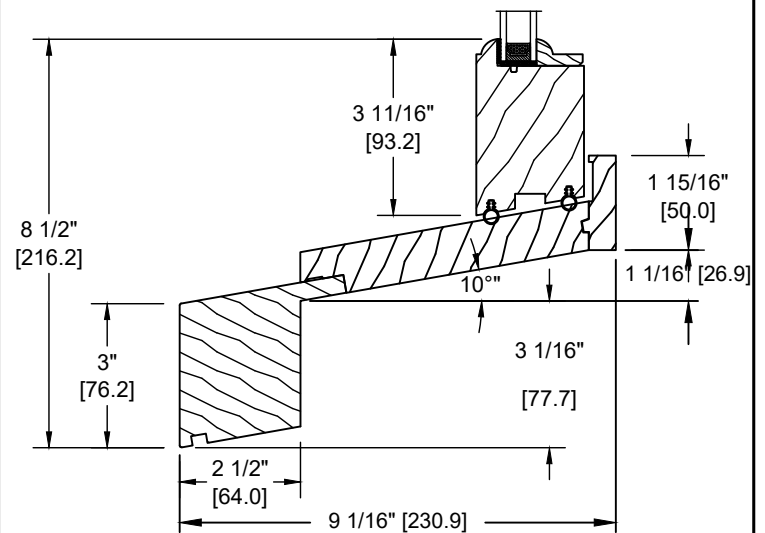
SPECIAL SILL EXTENSION (DS-073)
