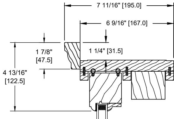
COLONIAL EXTERIOR BRICKMOULD (D-107)
