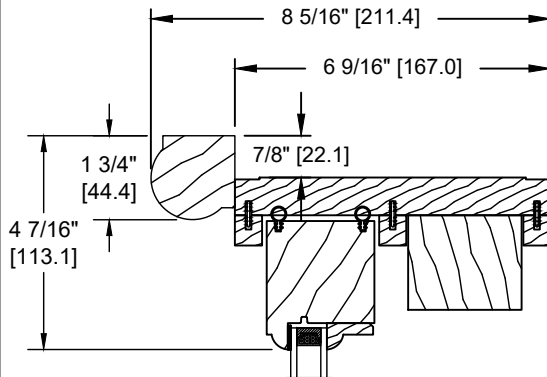
SPECIAL BRICKMOULD (DS-030)
