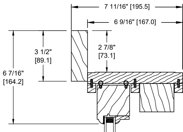
5/4 X 3 1/2" FLAT CASING (D-061)
