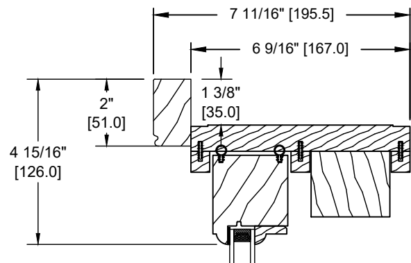
SPECIAL BRICKMOULD (DS-031)
