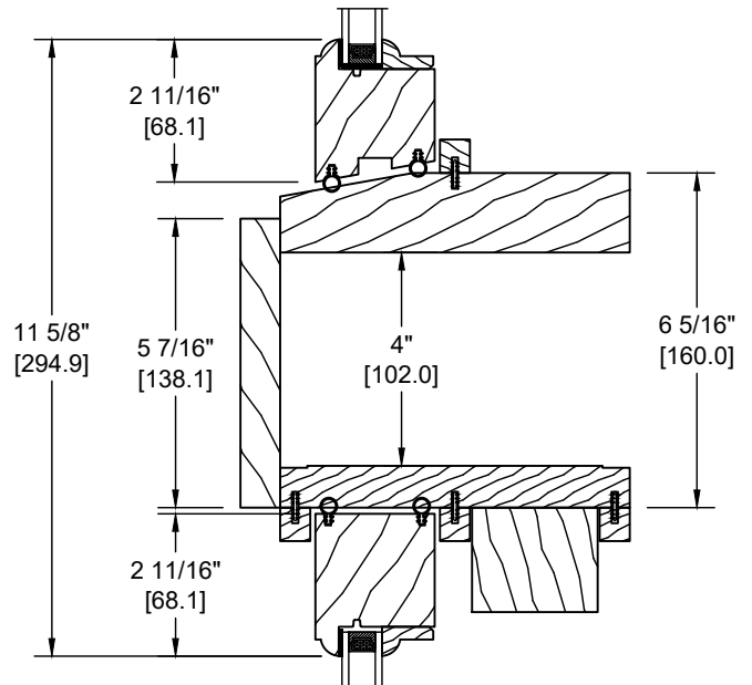
4" SPACE MULL OR STUD POCKET
