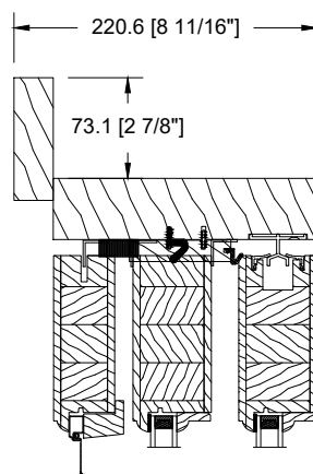
3 1/2" FLAT CASING
