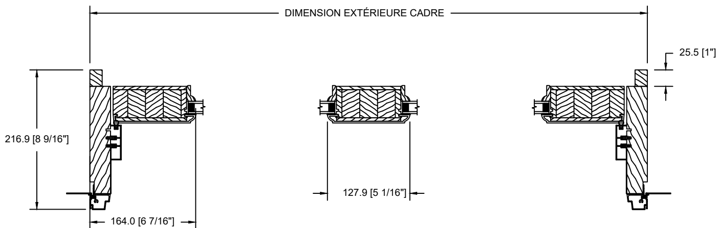
SECTION BB
