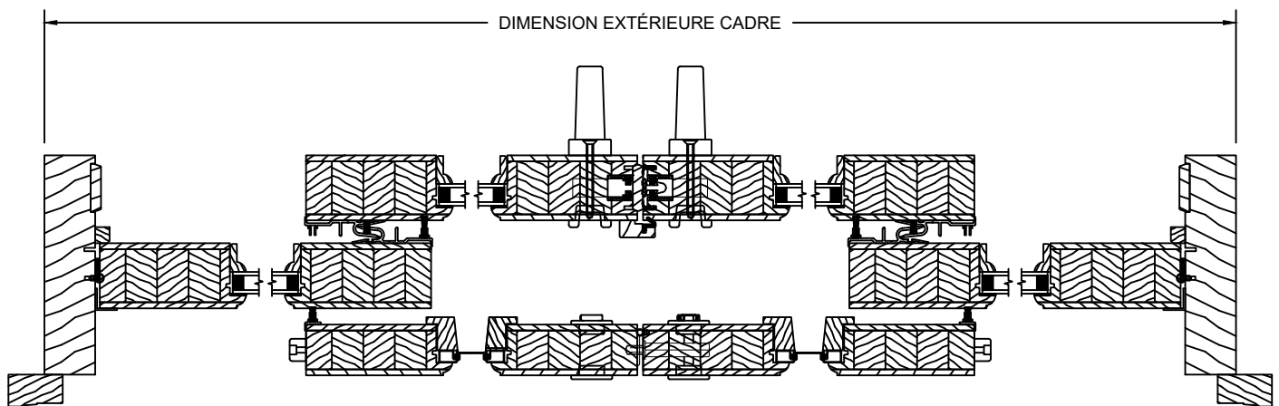
SECTION BB
