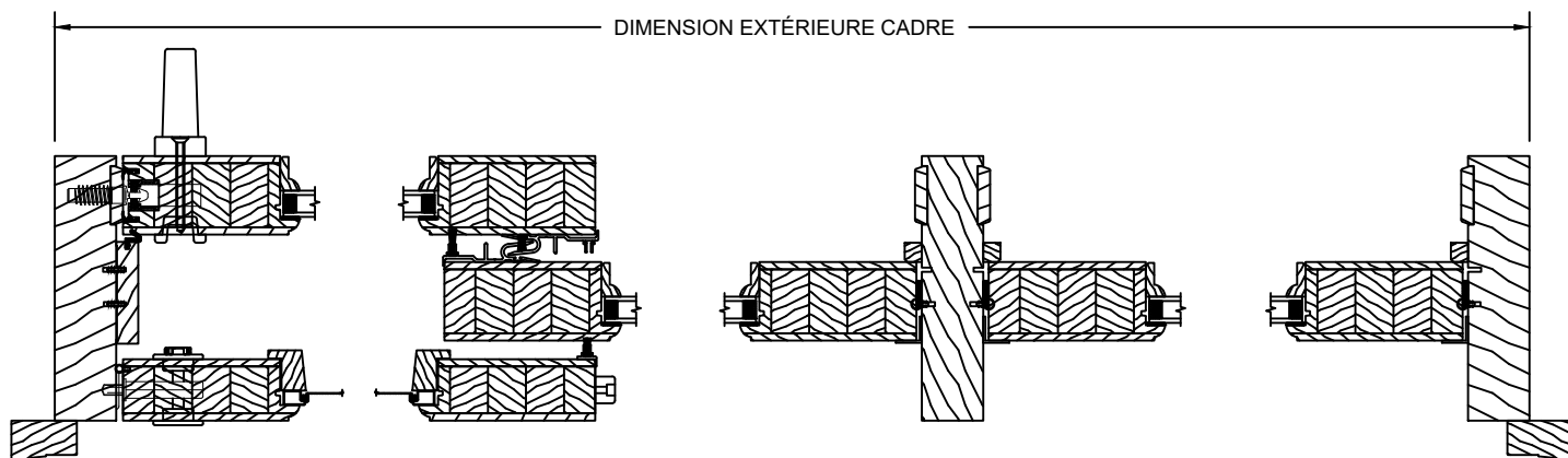
SECTION CC
