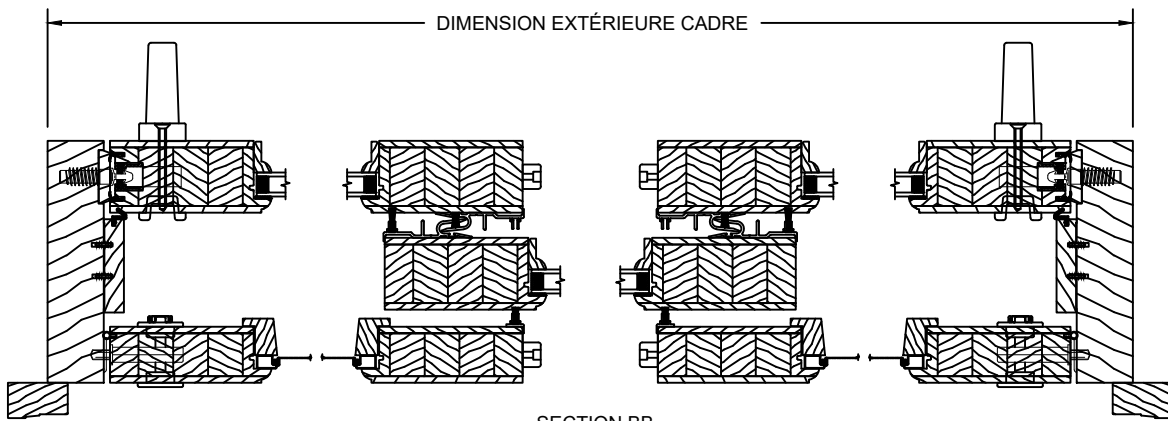
SECTION BB
