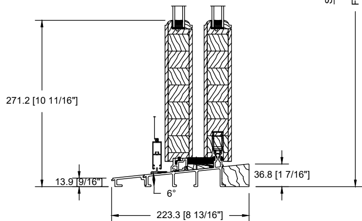
SECTION AA FRAME SIZE
