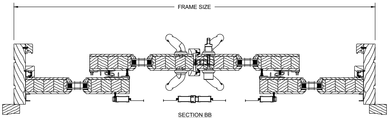
SECTION BB
