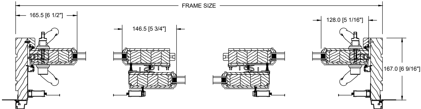
SECTION BB
