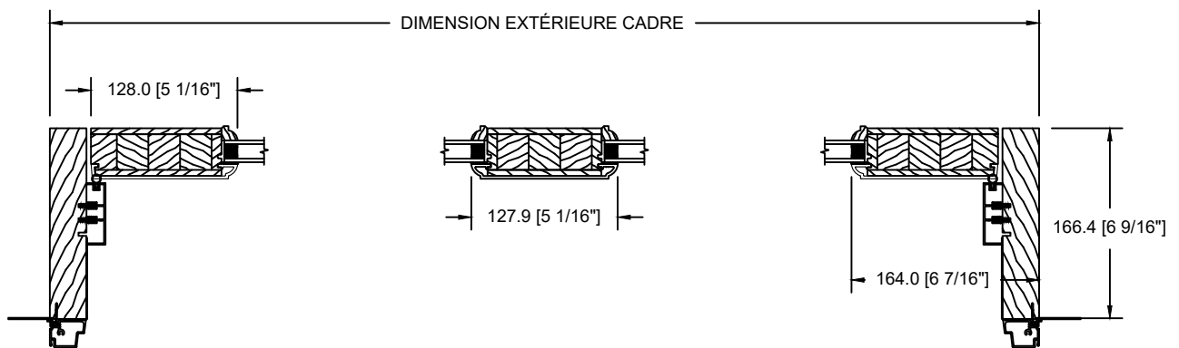
SECTION BB
