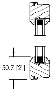
COLONIAL SASH & GLASS STOP
