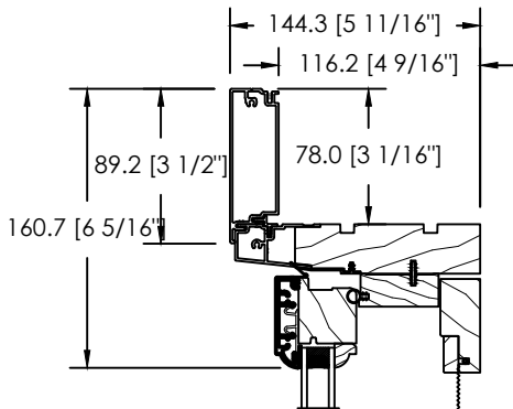
ALUMINIUM CLAD BACK BEND BRICKMOULD D-090
