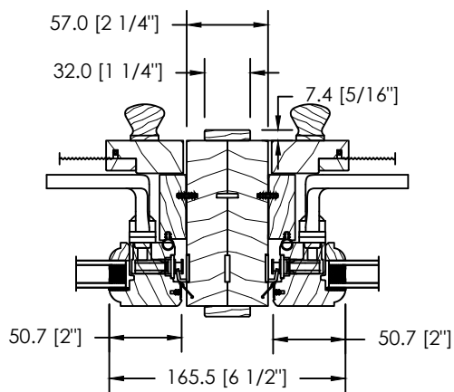
2 WIDE OPERATING STANDARD MODULAR MULL
