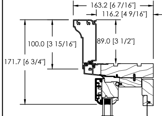
ALUMINIUM CLAD 3 1/2" FLAT BRICKMOULD D-050
