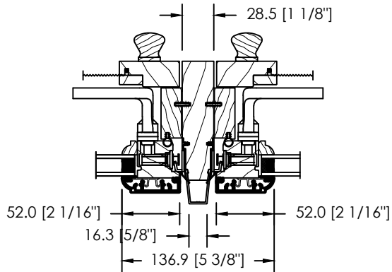
2 WIDE OPERATING STANDARD STRUCTURAL MULL
