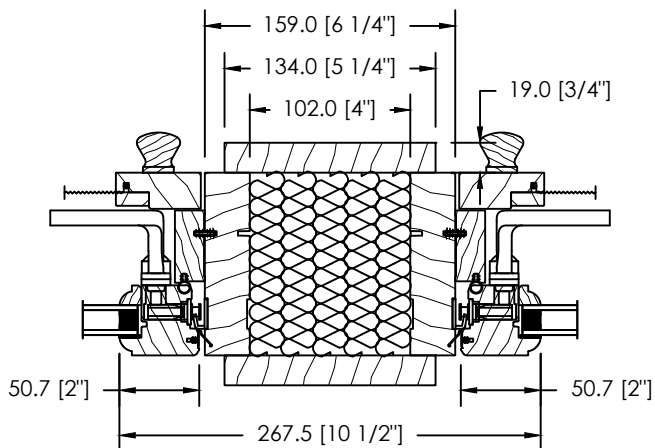
4" INSULATED SPACE MULL OR STUD POCKET
