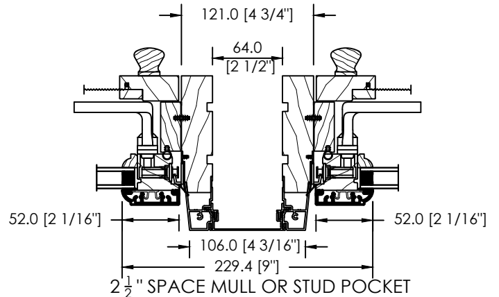
OPERATING, DIRECT SET MODULAR MULL
