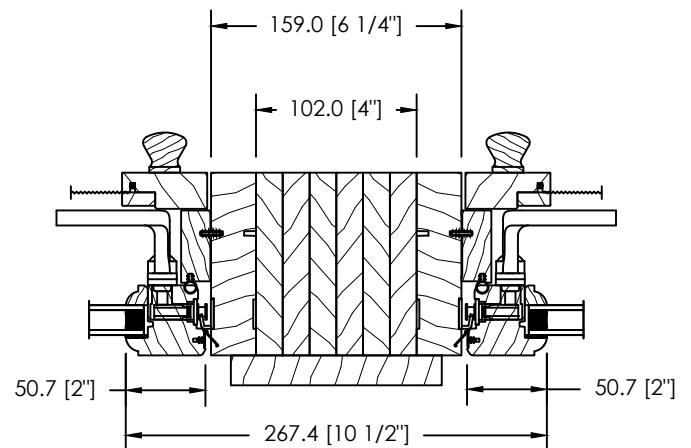
4" SOLID SPACE MULL OR STUD POCKET
