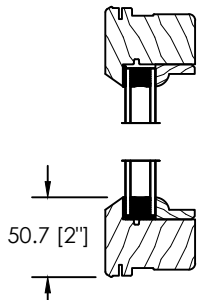
PUTTY GLAZE SASH & COLONIAL GLASS STOP
