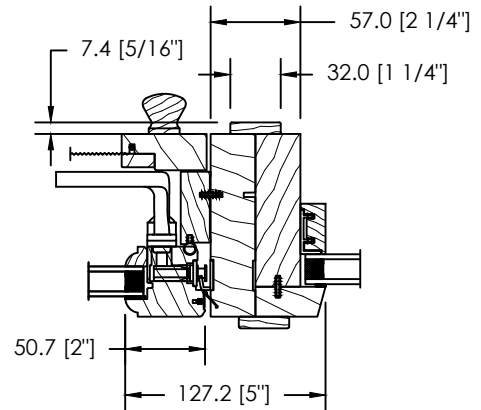
OPERATING, DIRECT SET MODULAR MULL
