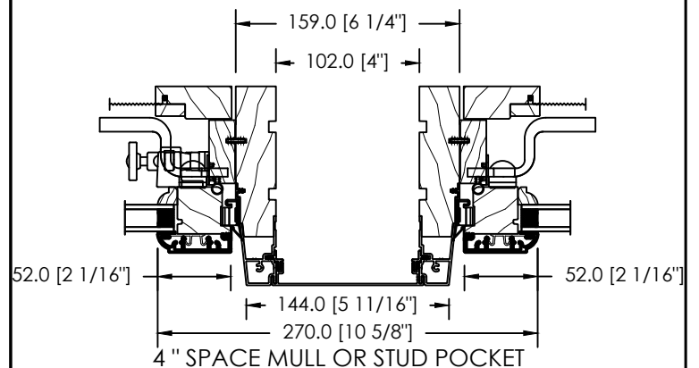
2 1/2" INSULATED SPACE MULL OR STUD POCKET
