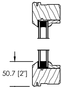
PUTTY GLAZE SASH & COLONIAL GLASS STOP
