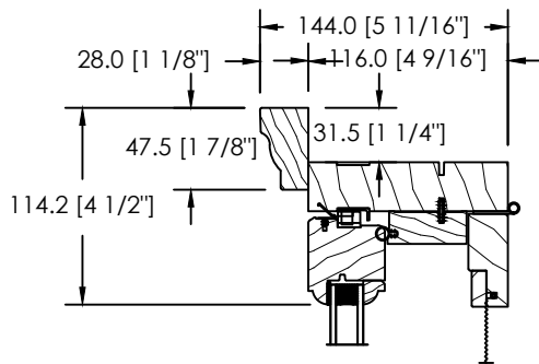
COLONIAL EXTERIOR BRICKMOULD
