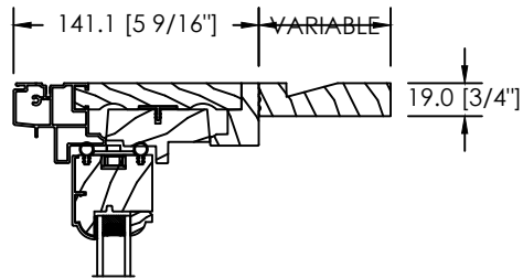
UP TO 3" INTERIOR EXTENSION
