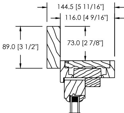
5/4 X 3 1/2" FLAT CASING (D-061)
