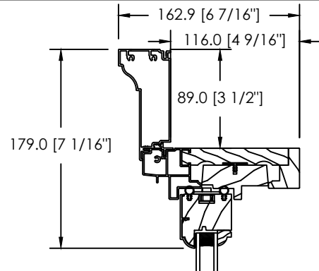
ALUMINIUM CLAD BACK BEND BRICKMOULD
