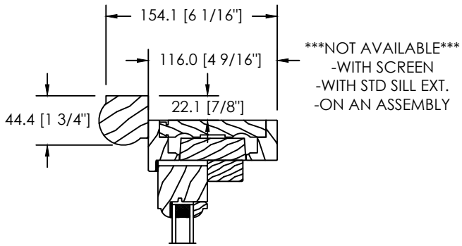
SPECIAL BRICKMOULD (DS-030)
