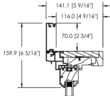
ALUMINIUM CLAD 2 3/4" FLAT BRICKMOULD
