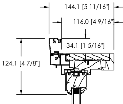
ALUMINIUM CLAD 908 BRICKMOULD
