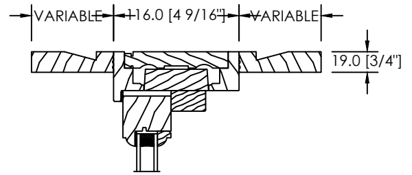
FLUSH UP TO 3" EXT. AND INT. EXTENSION
