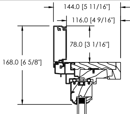
ALUMINIUM CLAD 3 1/2" FLAT BRICKMOULD
