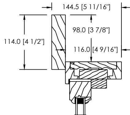
5/4 X 4 1/2" FLAT CASING (D-117)
