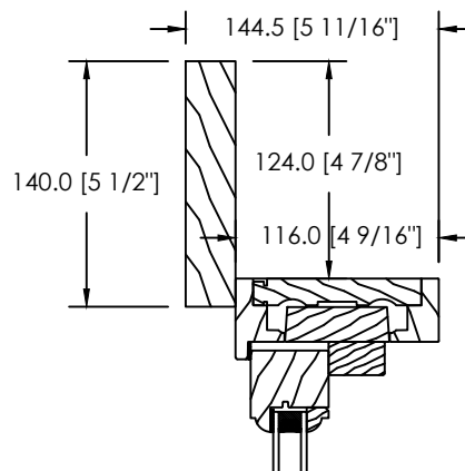
5/4 X 5 1/2" FLAT CASING (D-118)
