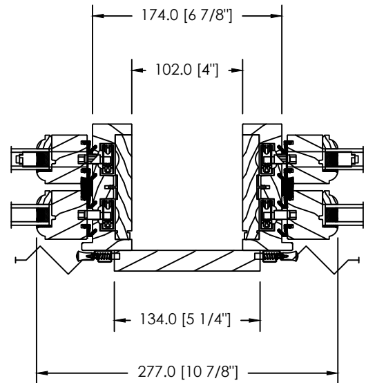
4" SPACE MULL OR STUD POCKET
