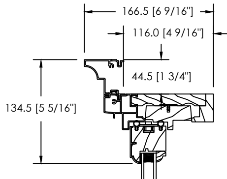
ALUMINIUM CLAD SKYLER BRICKMOULD
