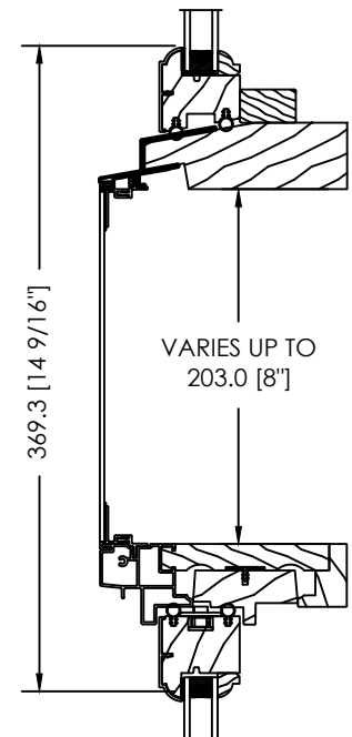
UP TO 8" SPACE MULL OR STUD POCKET
