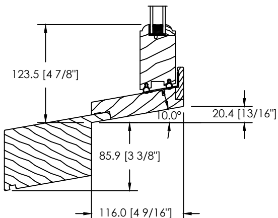
SPECIAL SILL EXTENSION (DS-072)
