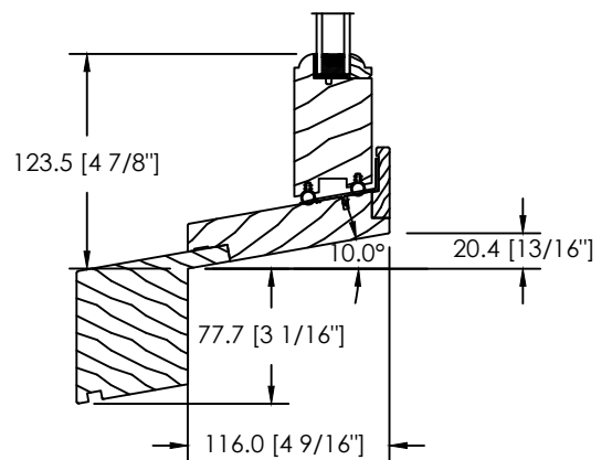
SPECIAL SILL EXTENSION (DS-073)
