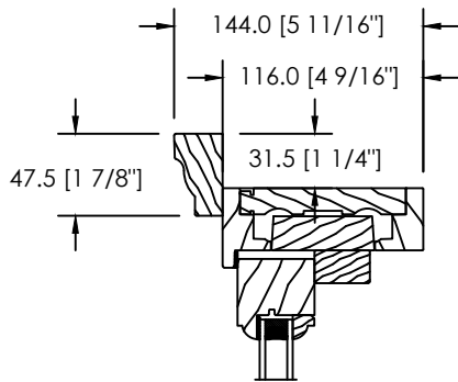
COLONIAL EXTERIOR BRICKMOULD (D-017)
