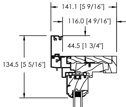
ALUMINIUM CLAD 1 3/4" FLAT BRICKMOULD
