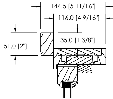
SPECIAL BRICKMOULD (DS-031)
