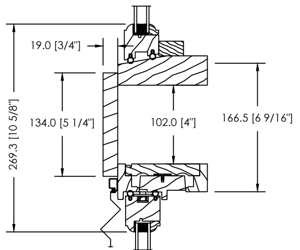
4" SPACE MULL OR STUD POCKET
