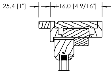
FLUSH 1" EXTERIOR EXTENSION
