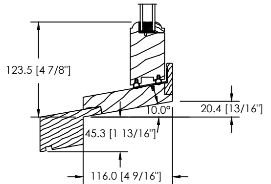
HISTORIC SILL EXTENSION (GB-036)
