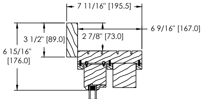
5/4 X 3 1/2" FLAT CASING (D-061)
