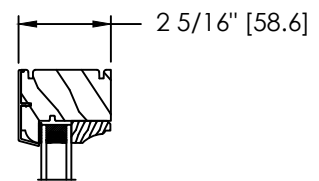
PUTTY GLAZE SASH & SQUARE GLASS STOP
