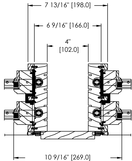
4" SPACE MULL OR STUD POCKET
