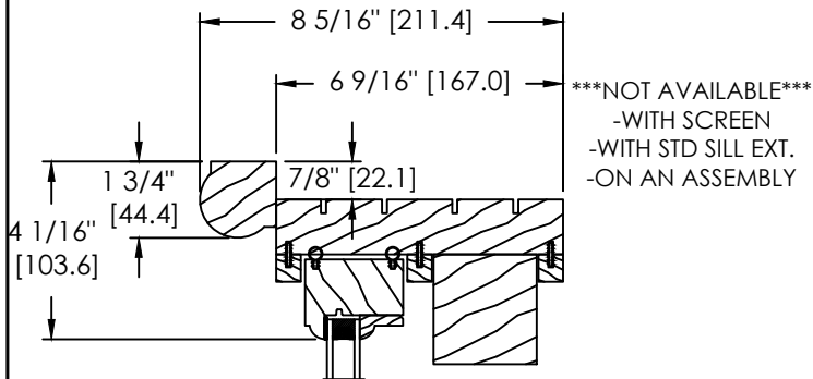
SPECIAL BRICKMOULD (DS-030)
