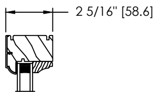
COLONIAL SASH & SQUARE GLASS STOP
