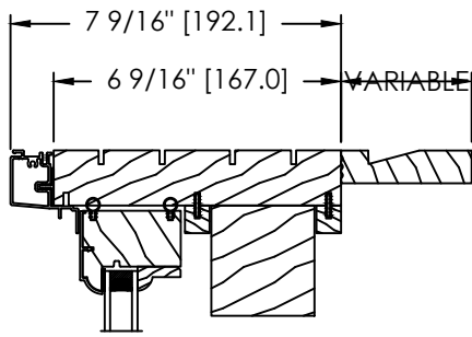
UP TO 3" INTERIOR EXTENSION
