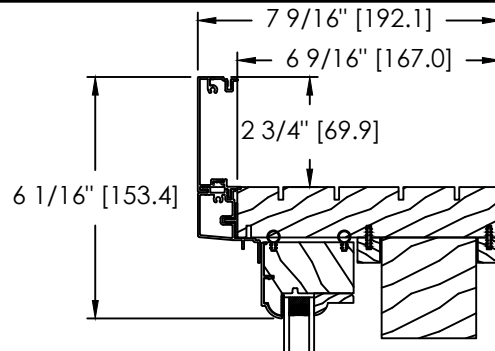
ALUMINIUM CLAD 2 3/4" FLAT BRICKMOULD
