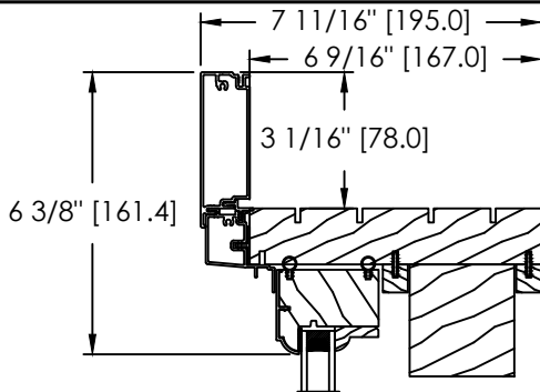
ALUMINIUM CLAD 3 1/2" FLAT BRICKMOULD
