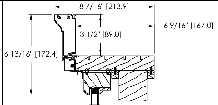
ALUMINIUM CLAD BACK BEND BRICKMOULD
