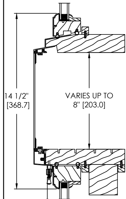
UP TO 8" SPACE MULL OR STUD POCKET
