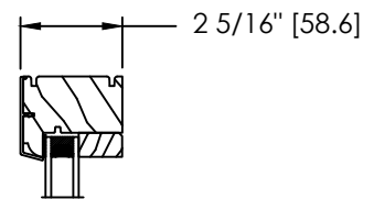
PUTTY GLAZE SASH & COLONIAL GLASS STOP
