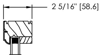
COLONIAL SASH & GLASS STOP
