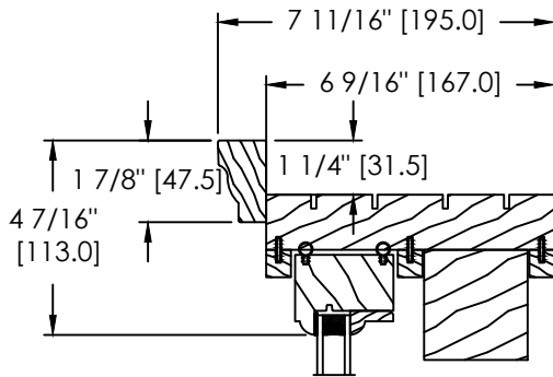
COLONIAL EXTERIOR BRICKMOULD (D-017)
