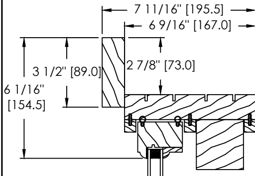
5/4 X 3 1/2" FLAT CASING (D-061)
