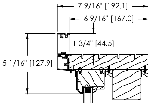
ALUMINIUM CLAD 1 3/4" FLAT BRICKMOULD
