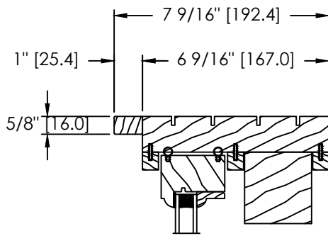
FLUSH 1" EXTERIOR EXTENSION
