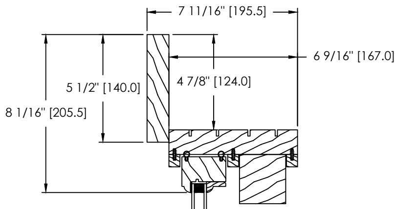
5/4 X 5 1/2" FLAT CASING (D-118)
