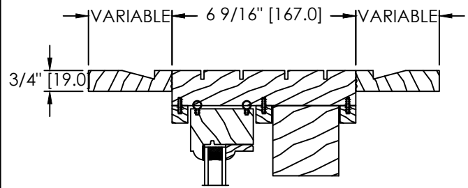
FLUSH UP TO 3" EXT. AND INT. EXTENSION
