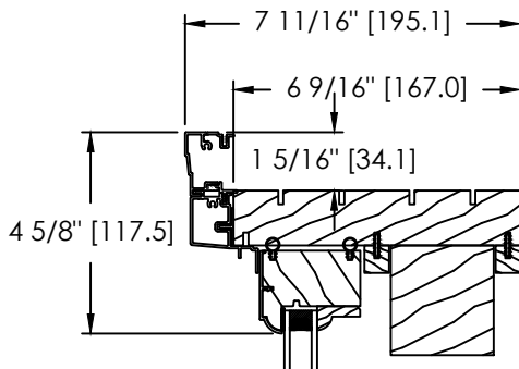
ALUMINIUM CLAD 908 BRICKMOULD
