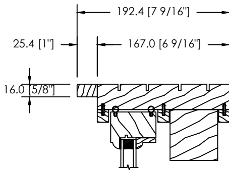
EXTENSION UNIE 25MM
