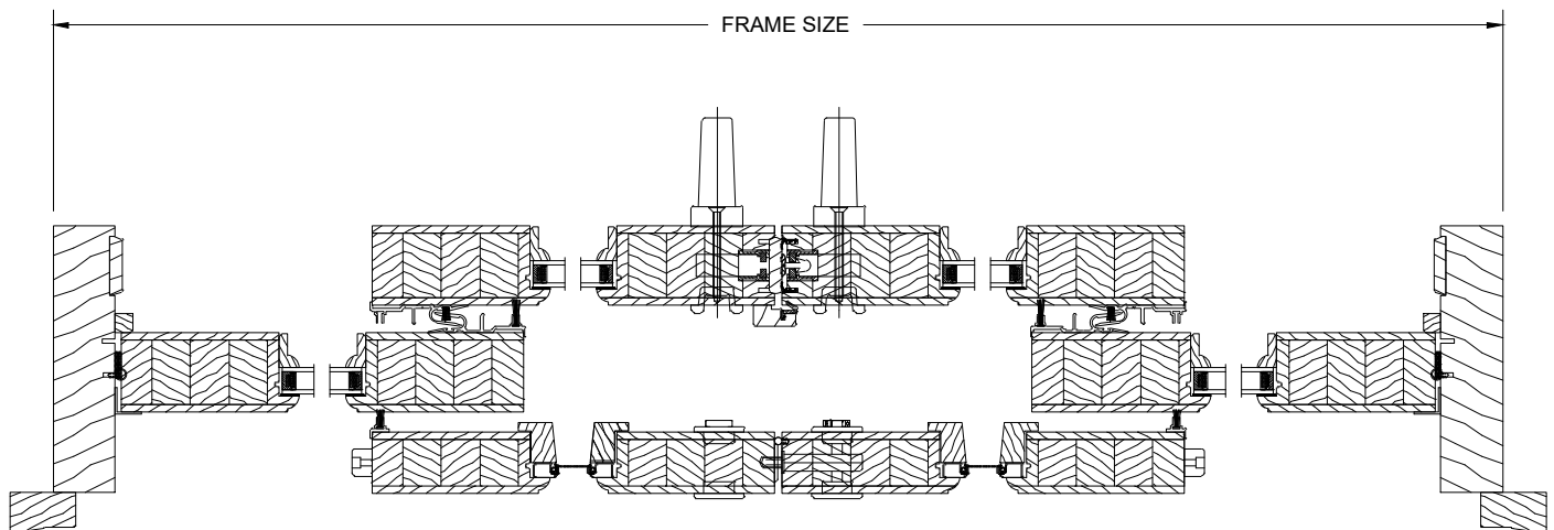
SECTION BB
