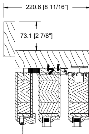
3 1/2" FLAT CASING
