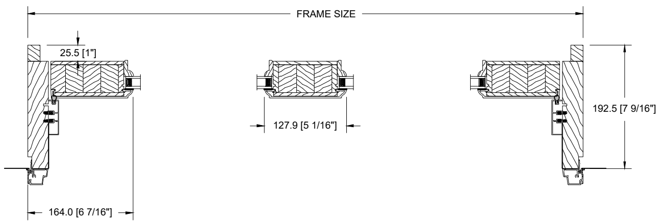
SECTION BB
