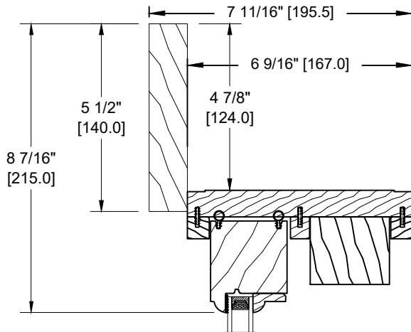
5/4 X 5 1/2" FLAT CASING (D-118)
