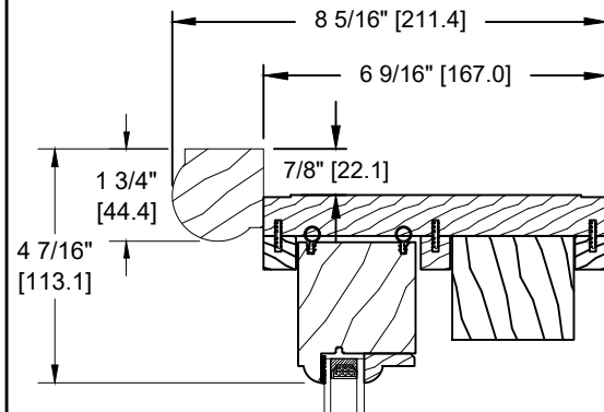
SPECIAL BRICKMOULD (DS-030)
