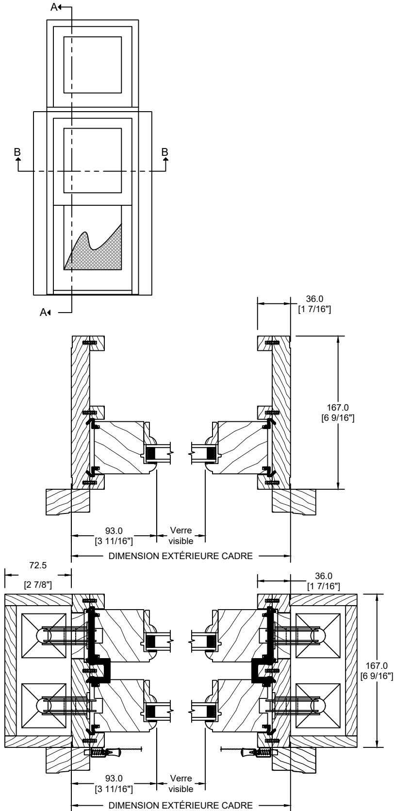
SECTION BB
