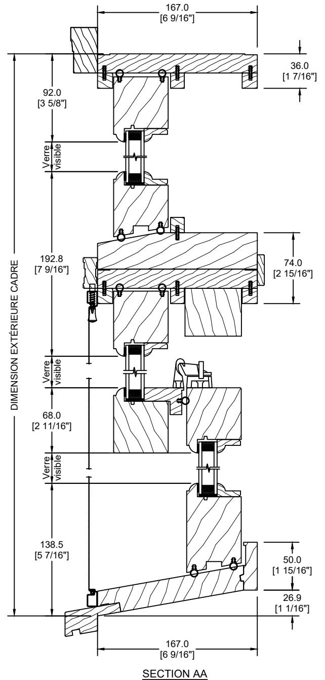
SECTION AA
