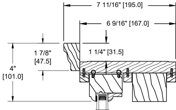
FLUSH 1" EXTERIOR EXTENSION
