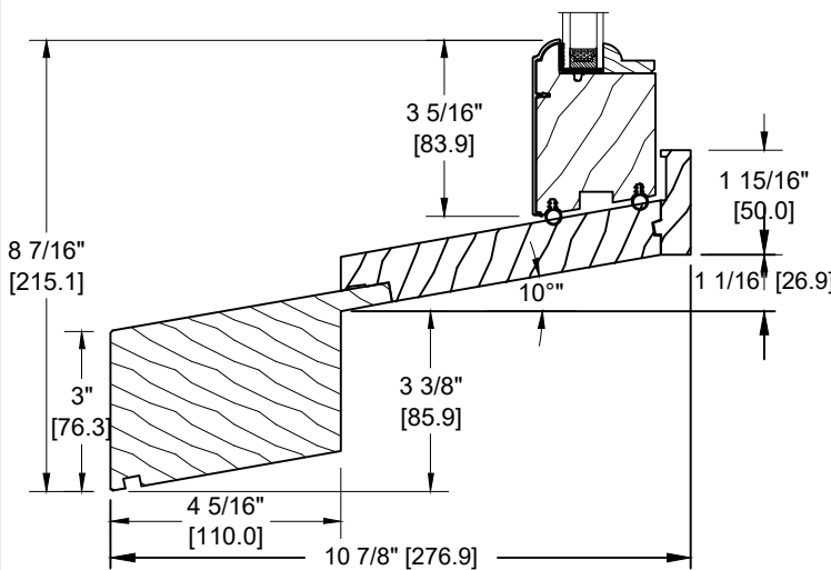
SPECIAL SILL EXTENSION (DS-072)
