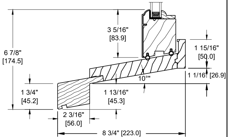
HISTORIC SILL EXTENSION (GB-036)
