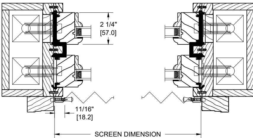
HALF SCREEN OPTION
