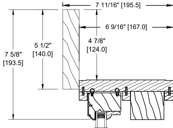
5/4 X 5 1/2" FLAT CASING (D-118)
