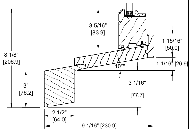
SPECIAL SILL EXTENSION (DS-073)
