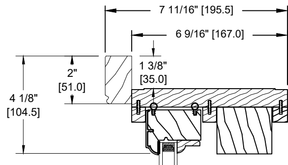
SPECIAL BRICKMOULD (DS-030)
