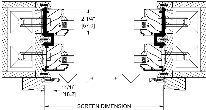
STANDARD SCREEN
