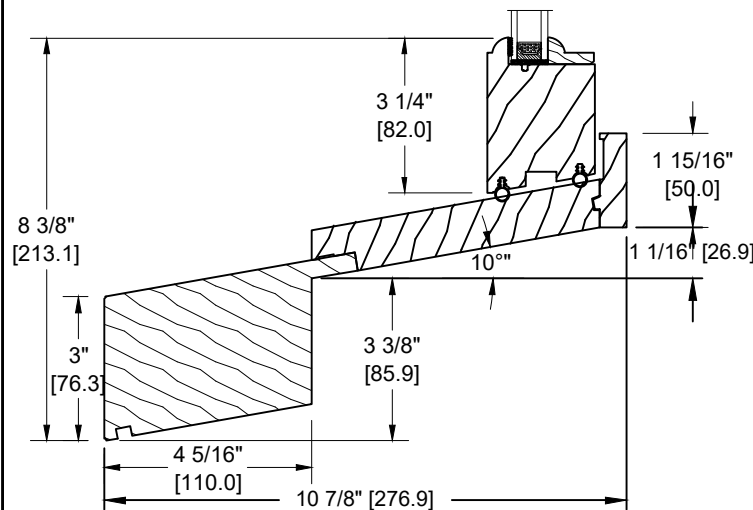
SPECIAL SILL EXTENSION (DS-072)
