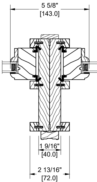
FIXED SASH MODULAR
