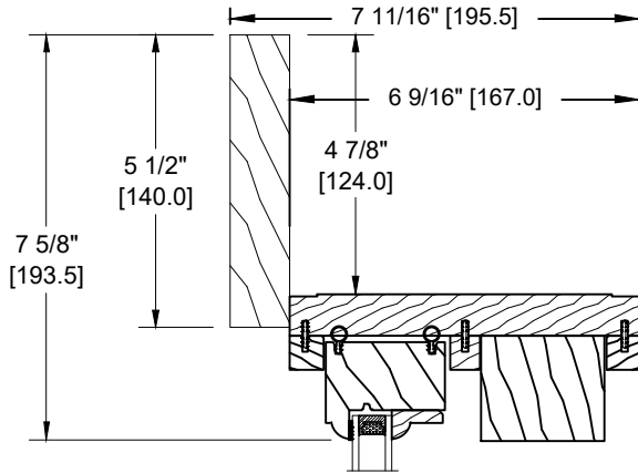
5/4 X 5 1/2" FLAT CASING (D-118)
