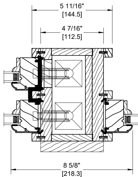
OPERATING WITH FIXED SASH MODULAR MULL
