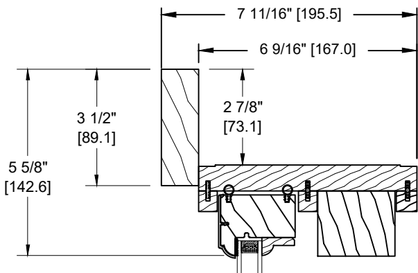
COLONIAL EXTERIOR BRICKMOULD (D-107)
