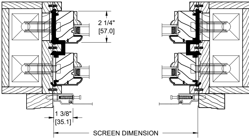
EXTRUDED SCREEN
