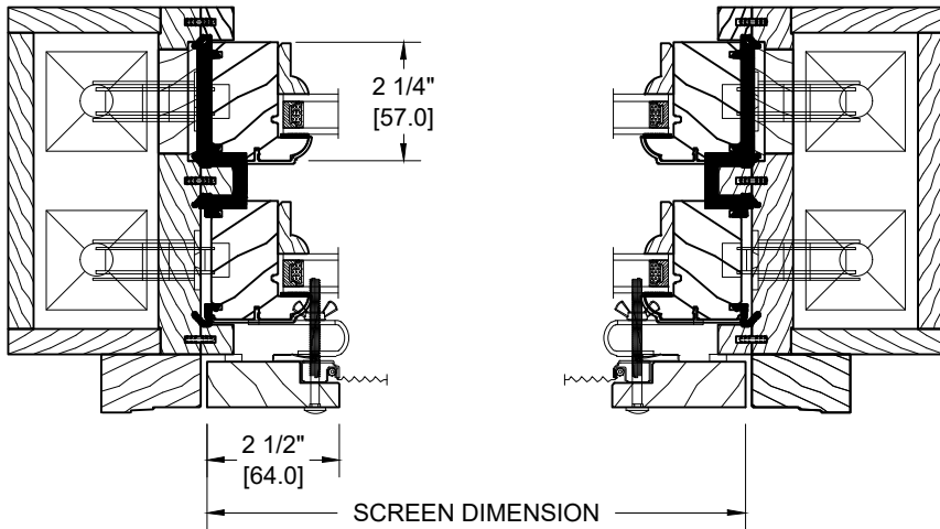
WOOD SCREEN OPTION
