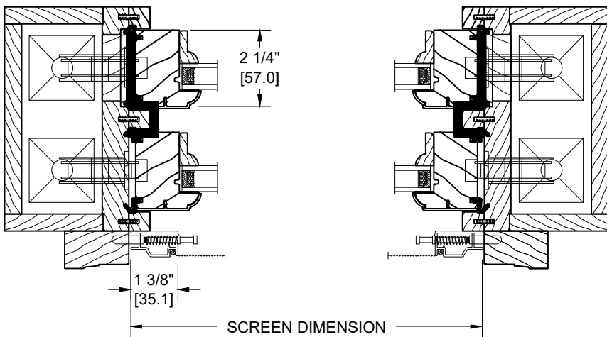
HALF EXTRUDED SCREEN OPTION
