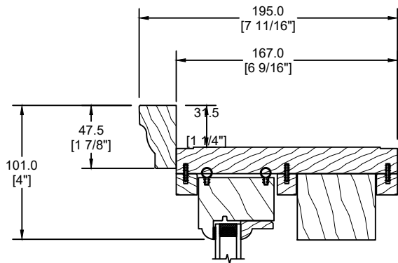
EXTENSION UNIE 25MM
