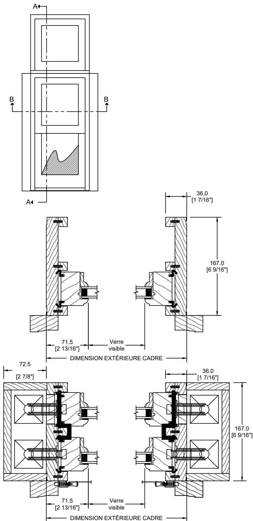
SECTION BB
