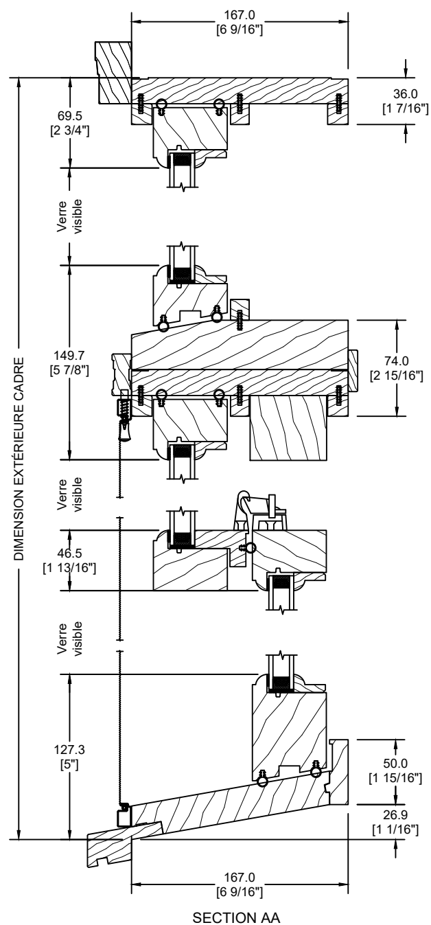
SECTION AA
