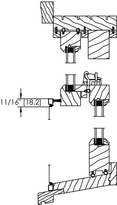
HALF SCREEN OPTION
