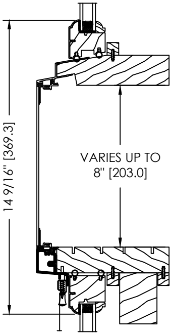
UP TO 8" SPACE MULL OR STUD POCKET
