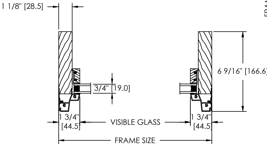
SECTION C - C
