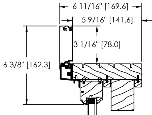
ALUMINIUM CLAD 3 1/2" FLAT BRICKMOULD
