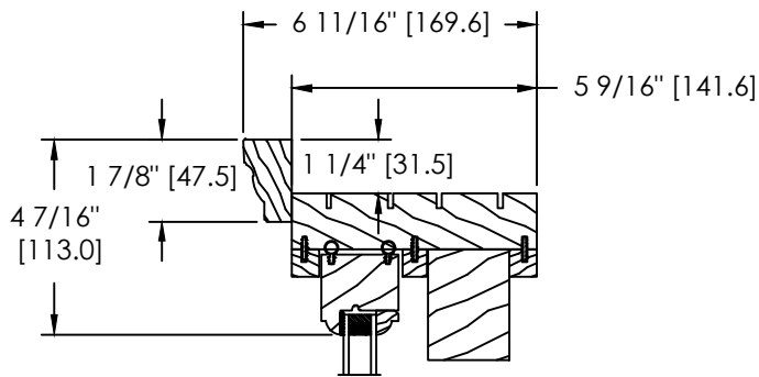
COLONIAL EXTERIOR BRICKMOULD (D-017)
