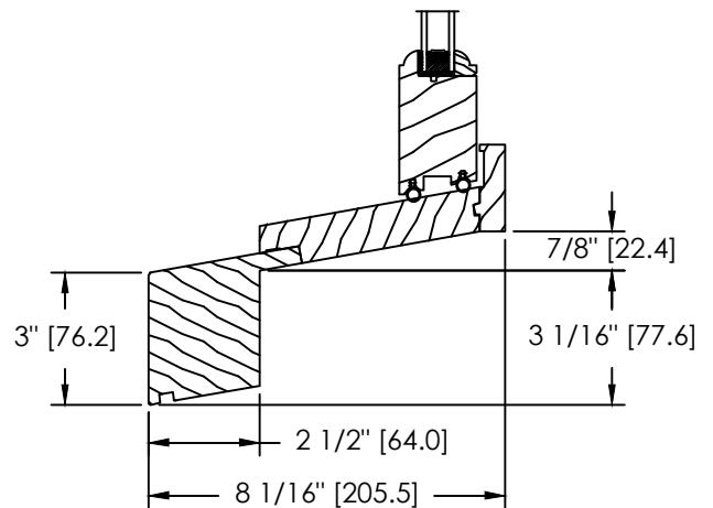
SPECIAL SILL EXTENSION (DS-073)
