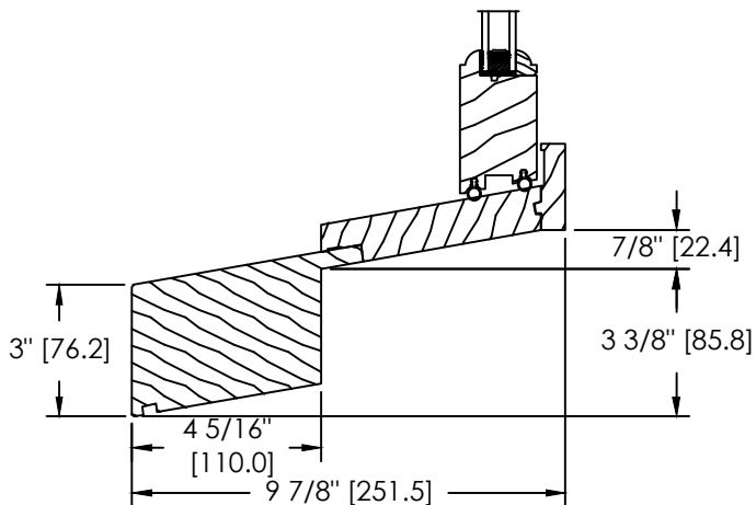
SPECIAL SILL EXTENSION (DS-072)
