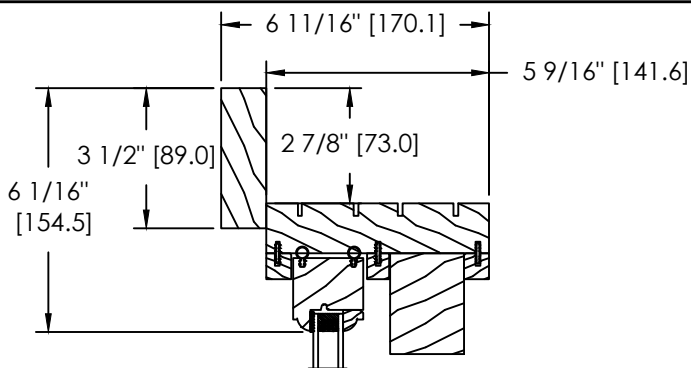
5/4 X 3 1/2" FLAT CASING (D-061)
