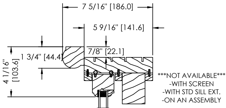
SPECIAL BRICKMOULD (DS-030)
