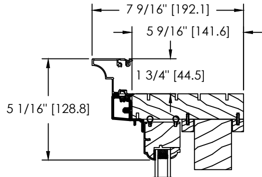
ALUMINIUM CLAD SKYLER BRICKMOULD
