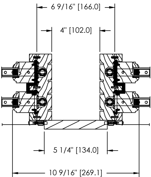
4" SPACE MULL OR STUD POCKET
