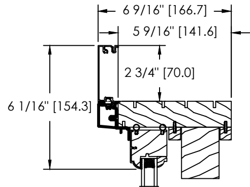
ALUMINIUM CLAD 2 3/4" FLAT BRICKMOULD
