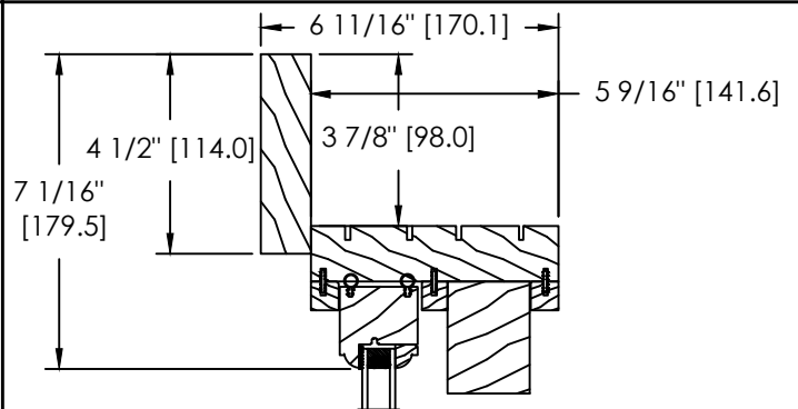
5/4 X 4 1/2" FLAT CASING (D-117)
