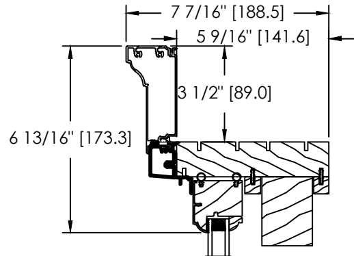
ALUMINIUM CLAD BACK BEND BRICKMOULD
