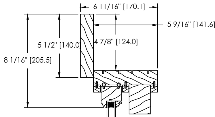
5/4 X 5 1/2" FLAT CASING (D-118)
