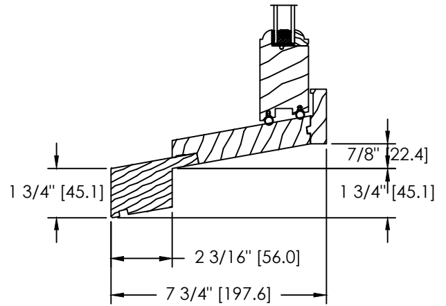
HISTORIC SILL EXTENSION (GB-036)
