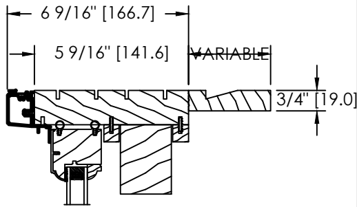
UP TO 3" INTERIOR EXTENSION
