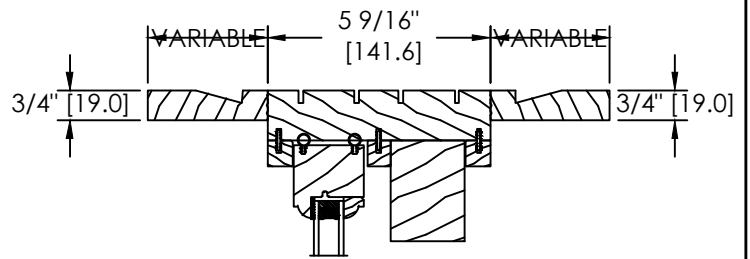
FLUSH UP TO 3" EXT. AND INT. EXTENSION
