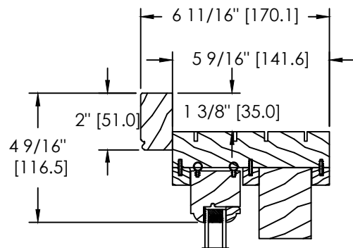
SPECIAL BRICKMOULD (DS-031)
