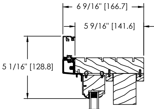
ALUMINIUM CLAD 1 3/4" FLAT BRICKMOULD
