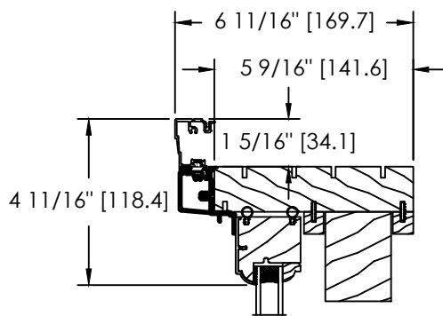
ALUMINIUM CLAD 908 BRICKMOULD
