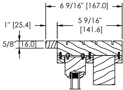
FLUSH 1" EXTERIOR EXTENSION
