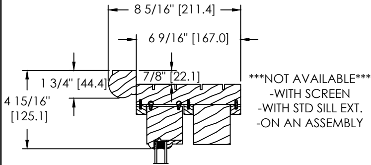
SPECIAL BRICKMOULD (DS-030)
