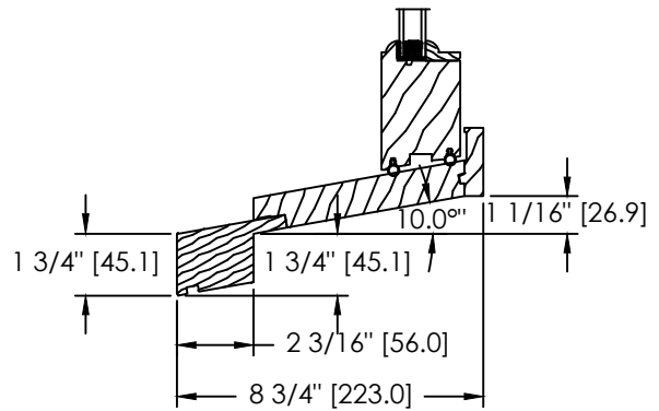
HISTORIC SILL EXTENSION (GB-036)
