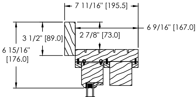
5/4 X 3 1/2" FLAT CASING (D-061)
