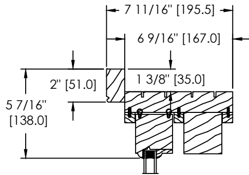
SPECIAL BRICKMOULD (DS-031)
