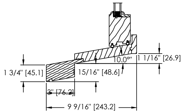
HISTORIC 3" SILL EXTENSION (GB-058)
