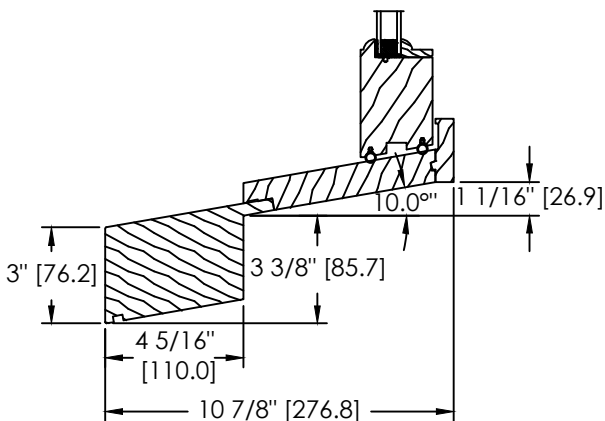
SPECIAL SILL EXTENSION (DS-072)
