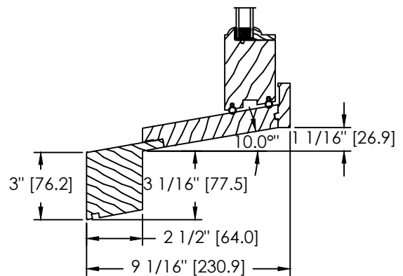
SPECIAL SILL EXTENSION (DS-073)
