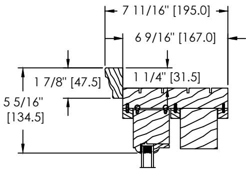
COLONIAL EXTERIOR BRICKMOULD (D-017)
