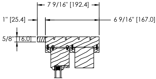
FLUSH 1" EXTERIOR EXTENSION
