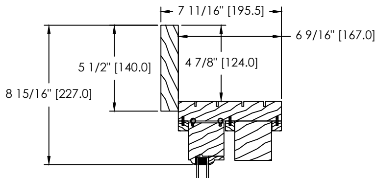
5/4 X 5 1/2" FLAT CASING (D-118)
