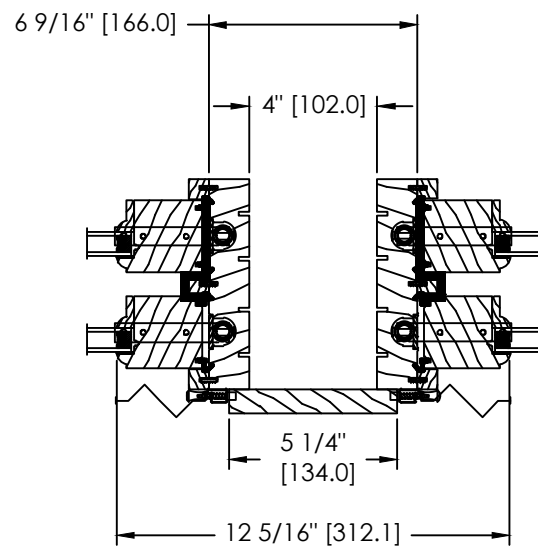
4" SPACE MULL OR STUD POCKET
