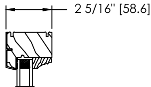
PUTTY GLAZE SASH & SQUARE GLASS STOP
