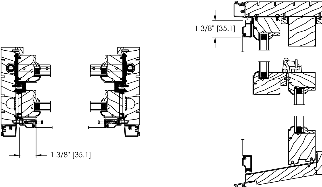
EXTRUDED SCREEN OPTION
