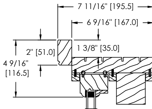
SPECIAL BRICKMOULD (DS-031)
