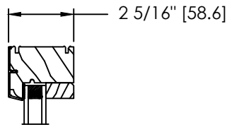
PUTTY GLAZE SASH & COLONIAL GLASS STOP
