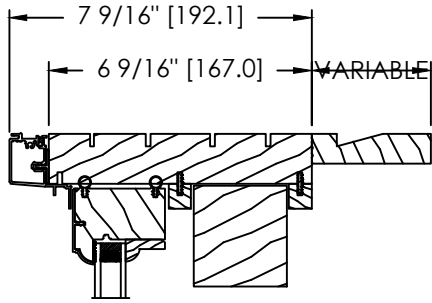
UP TO 3" INTERIOR EXTENSION
