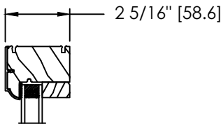
COLONIAL SASH & GLASS STOP
