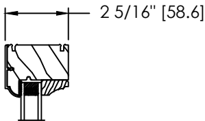
COLONIAL SASH & SQUARE GLASS STOP
