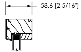
VOLET CONTEMPORAIN & PARECLOUSE COLONIAL
