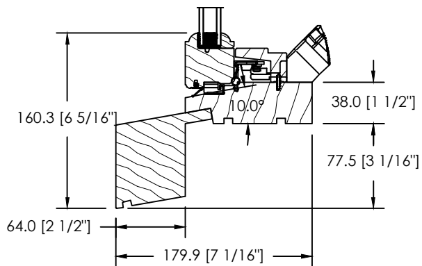
DS-073 SILL NOSING
