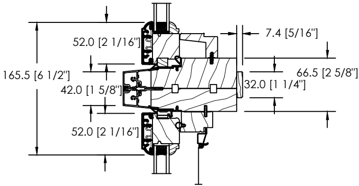
FIXED OVER OPERATING TIGHT MULL
