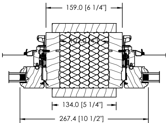
4" INSULATED SPACE MULL OR STUD POCKET
