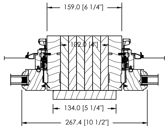
4" SOLID SPACE MULL OR STUD POCKET
