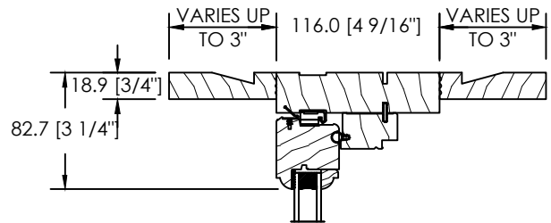
FLUSH UP TO 3" EXT. AND INT. EXTENSION
