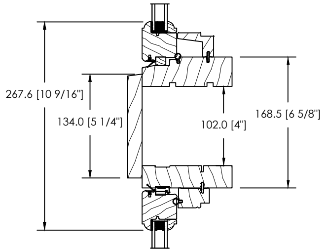
4" SPACE MULL OR STUD POCKET
