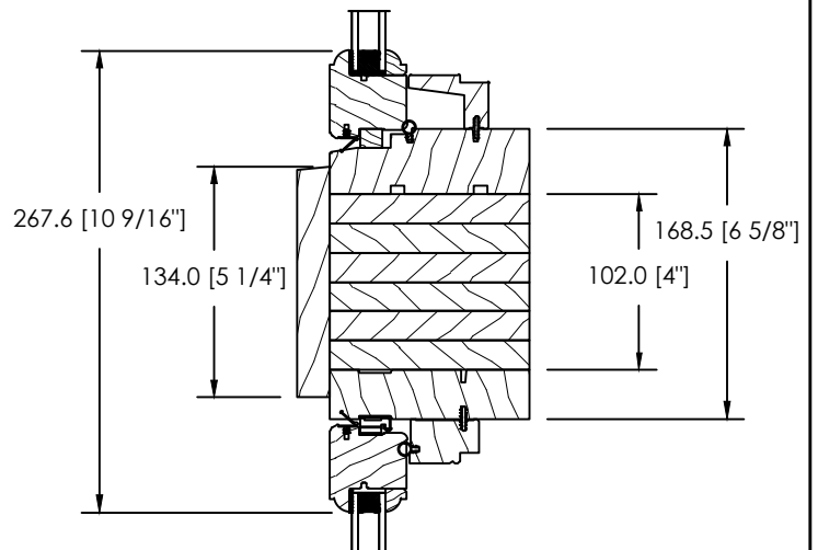
4" SOLID SPACE MULL OR STUD POCKET
