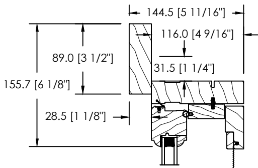
5/4 X 3 1/2" FLAT CASING
