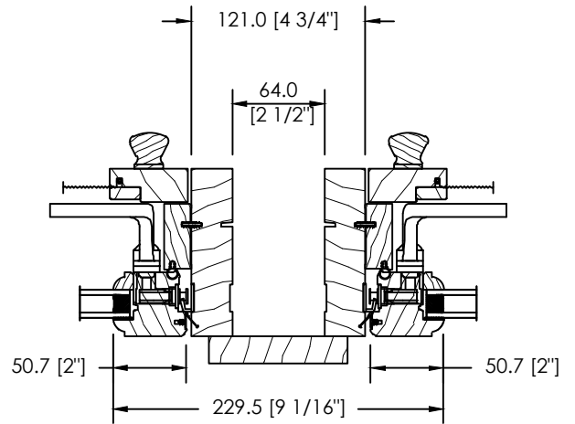
OPERATING, DIRECT SET MODULAR MULL
