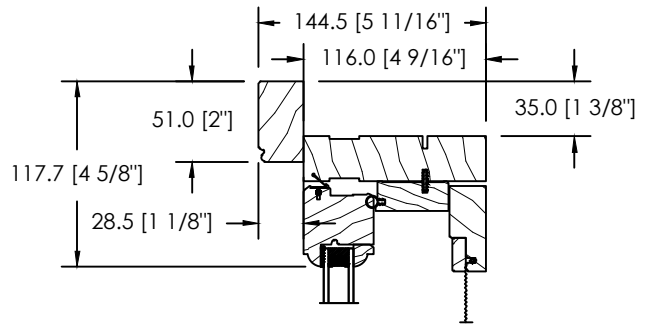
DS-031 BRICKMOULD
