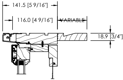
INTERIOR EXTENSION
