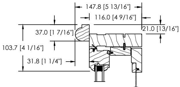
DS-034 BRICKMOULD
