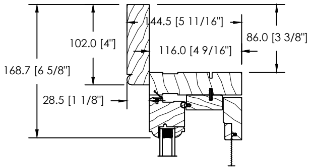
DS-001 BRICKMOULD
