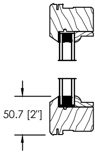
PUTTY GLAZE SASH & COLONIAL GLASS STOP
