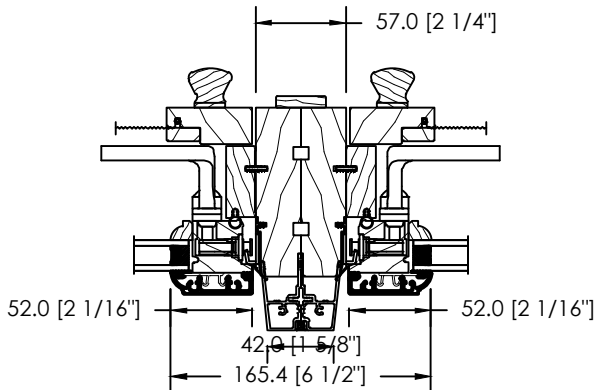
2 WIDE OPERATING STANDARD MODULAR MULL
