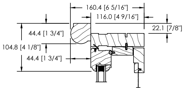
DS-030 BRICKMOULD
