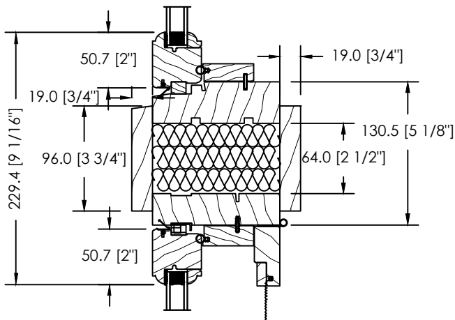
2 1/2" INSULATED SPACE MULL OR STUD POCKET
