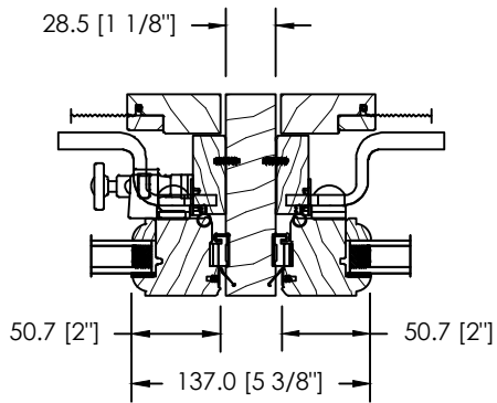
2 WIDE OPERATING STANDARD STRUCTURAL MULL
