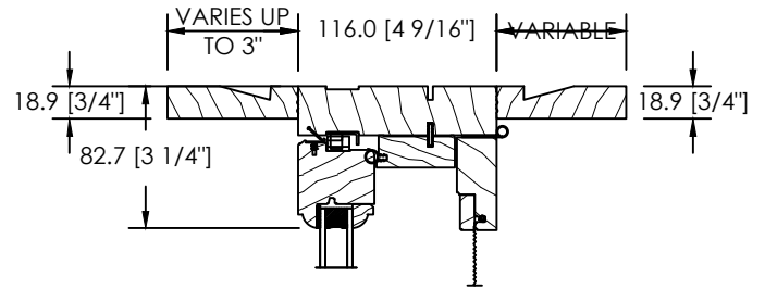
FLUSH UP TO 3" EXT. AND INT. EXTENSION
