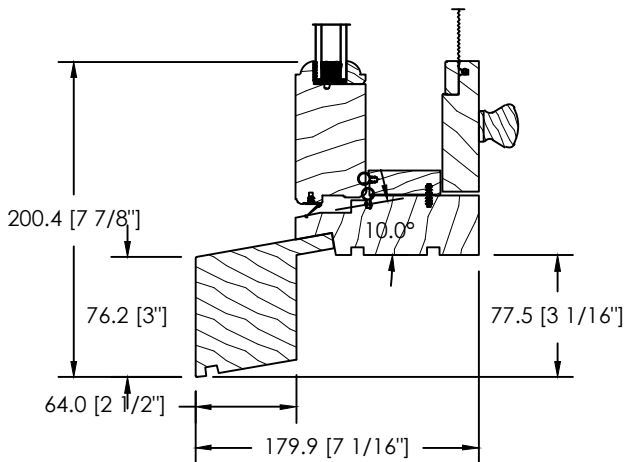
DS-073 SILL NOSING
