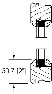
COLONIAL SASH & GLASS STOP
