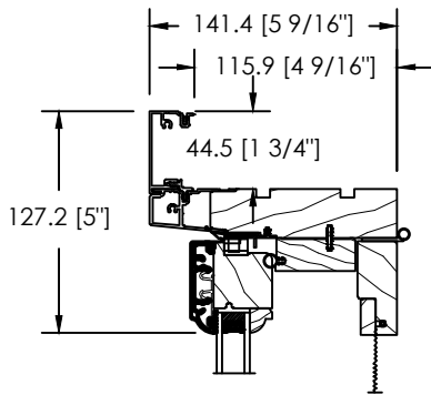
ALUMINIUM CLAD 1 3/4" FLAT BRICKMOULD D-116
