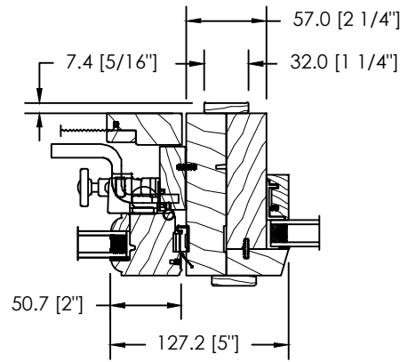
OPERATING, DIRECT SET MODULAR MULL
