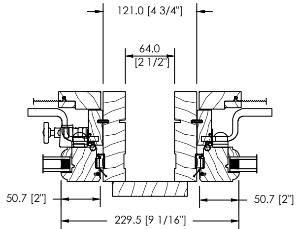
OPERATING, DIRECT SET MODULAR MULL
