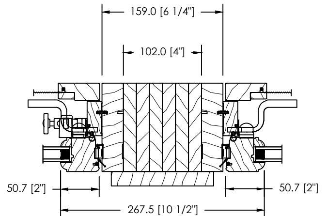
4" SOLID SPACE MULL OR STUD POCKET
