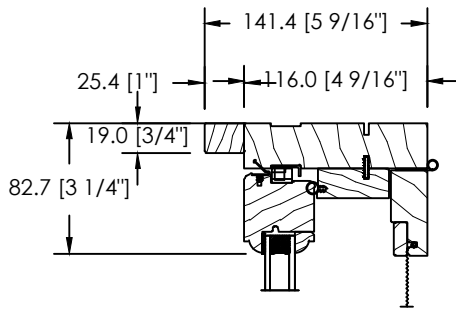
FLUSH 1" EXTERIOR EXTENSION
