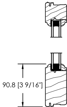
COLONIAL SASH & GLASS STOP-WIDE BOTTOM RAIL
