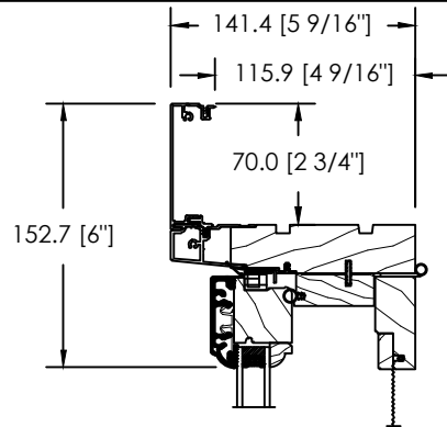
ALUMINIUM CLAD 2 3/4" FLAT BRICKMOULD D-066
