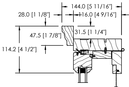
COLONIAL EXTERIOR BRICKMOULD
