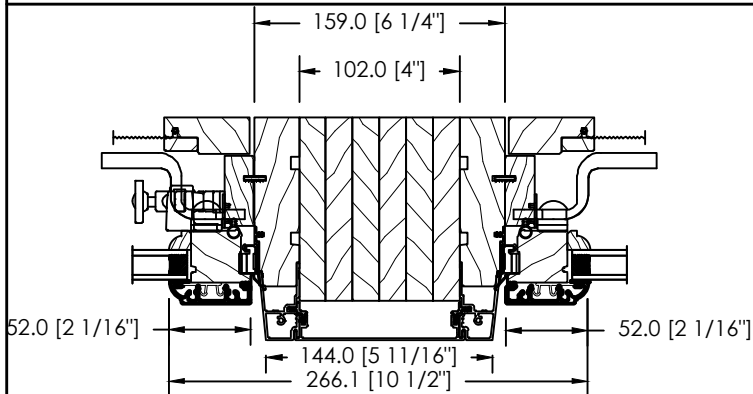
4" SOLID SPACE MULL OR STUD POCKET
