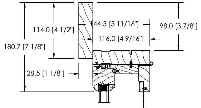
5/4 X 4 1/2" FLAT CASING
