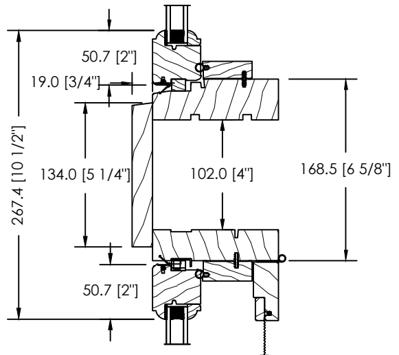
4" SPACE MULL OR STUD POCKET
