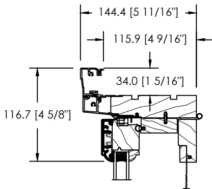
ALUMINIUM CLAD 908 BRICKMOULD
