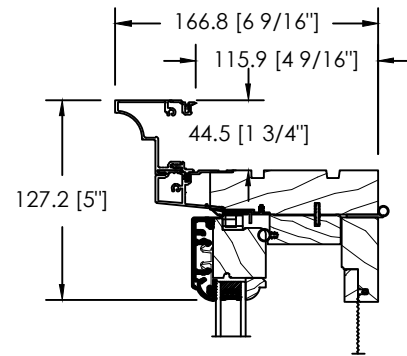
ALUMINIUM CLAD SKYLER BRICKMOULD D-174
