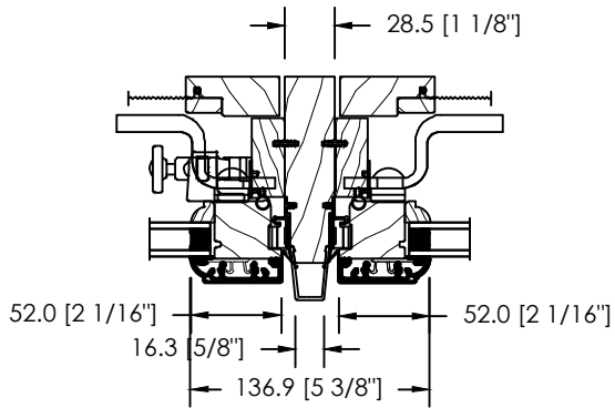
2 WIDE OPERATING STANDARD STRUCTURAL MULL
