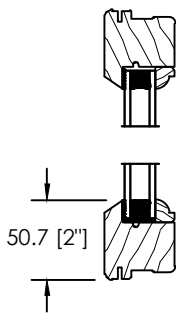
PUTTY GLAZE SASH & COLONIAL GLASS STOP
