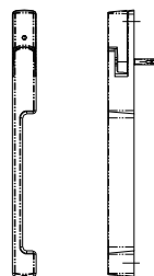
Q-277 Poignée Patio Prestige Dallas / Prestige Dallas Sliding Handle
